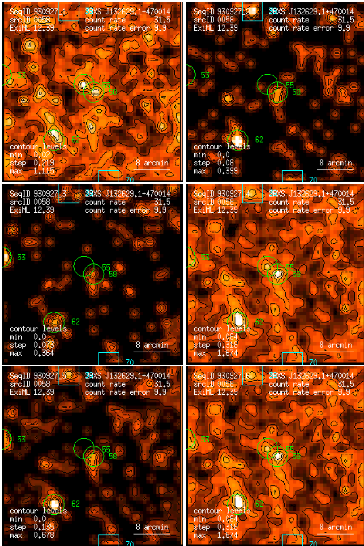
Figure 58: RASS 930927: detection 0058: band rate images, Gaussian filter: (1) PSPC channels 11 – 41, (2) 52 – 90, (3) 91 – 201, (4) 11 – 235, (5) 52 – 201, (6) 11 – 201. Broad band rates in counts/ks. Band rate contour levels in counts/ks/arcmin 2 .
