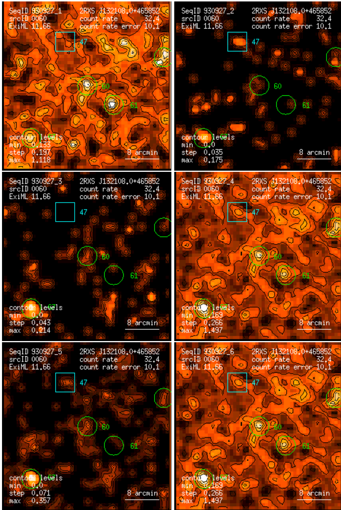
Figure 60: RASS 930927: detection 0060: band rate images, Gaussian filter: (1) PSPC channels 11 – 41, (2) 52 – 90, (3) 91 – 201, (4) 11 – 235, (5) 52 – 201, (6) 11 – 201. Broad band rates in counts/ks. Band rate contour levels in counts/ks/arcmin 2 .
