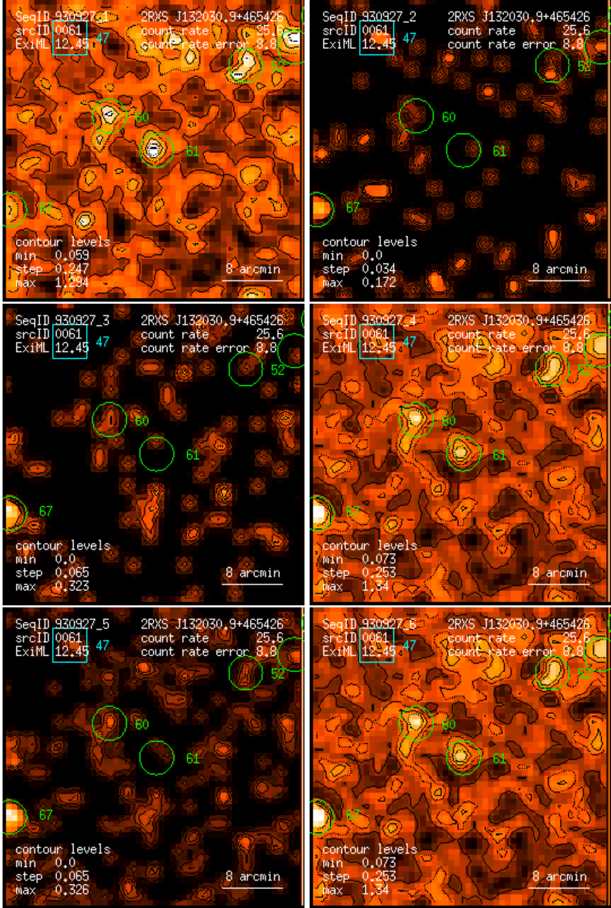
Figure 61: RASS 930927: detection 0061: band rate images, Gaussian filter: (1) PSPC channels 11 – 41, (2) 52 – 90, (3) 91 – 201, (4) 11 – 235, (5) 52 – 201, (6) 11 – 201. Broad band rates in counts/ks. Band rate contour levels in counts/ks/arcmin 2 .
