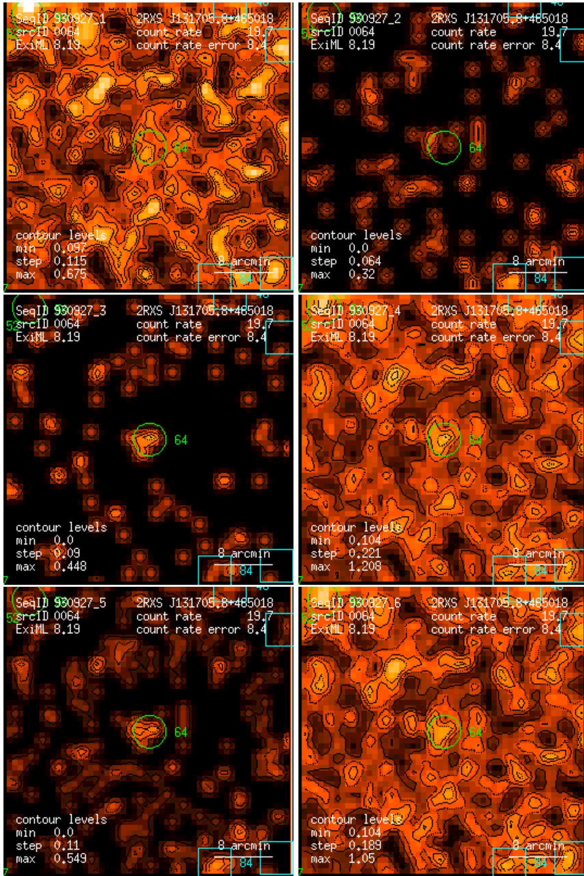
Figure 64: RASS 930927: detection 0064: band rate images, Gaussian filter: (1) PSPC channels 11 – 41, (2) 52 – 90, (3) 91 – 201, (4) 11 – 235, (5) 52 – 201, (6) 11 – 201. Broad band rates in counts/ks. Band rate contour levels in counts/ks/arcmin 2 .
