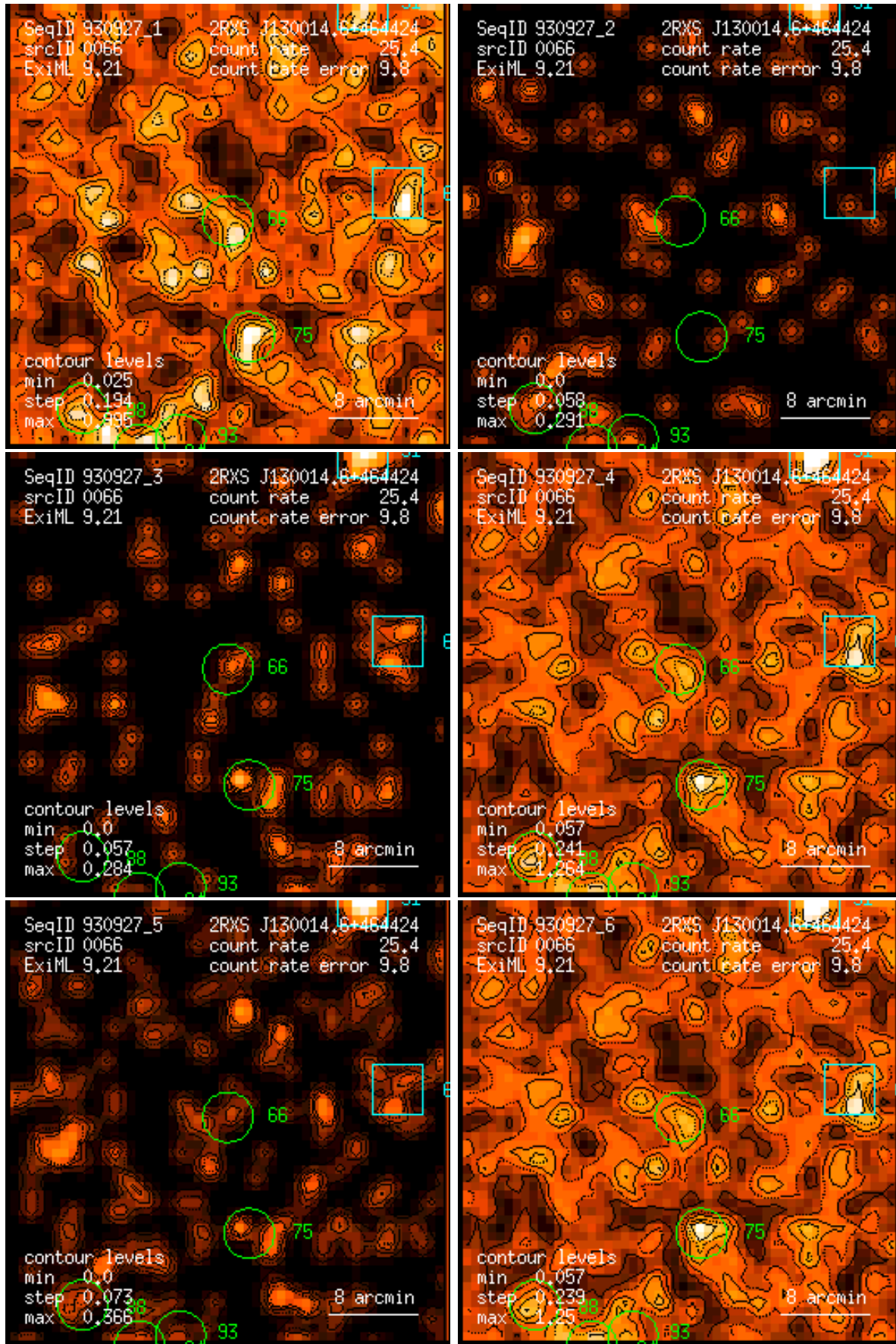
Figure 66: RASS 930927: detection 0066: band rate images, Gaussian filter: (1) PSPC channels 11 – 41, (2) 52 – 90, (3) 91 – 201, (4) 11 – 235, (5) 52 – 201, (6) 11 – 201. Broad band rates in counts/ks. Band rate contour levels in counts/ks/arcmin 2 .
