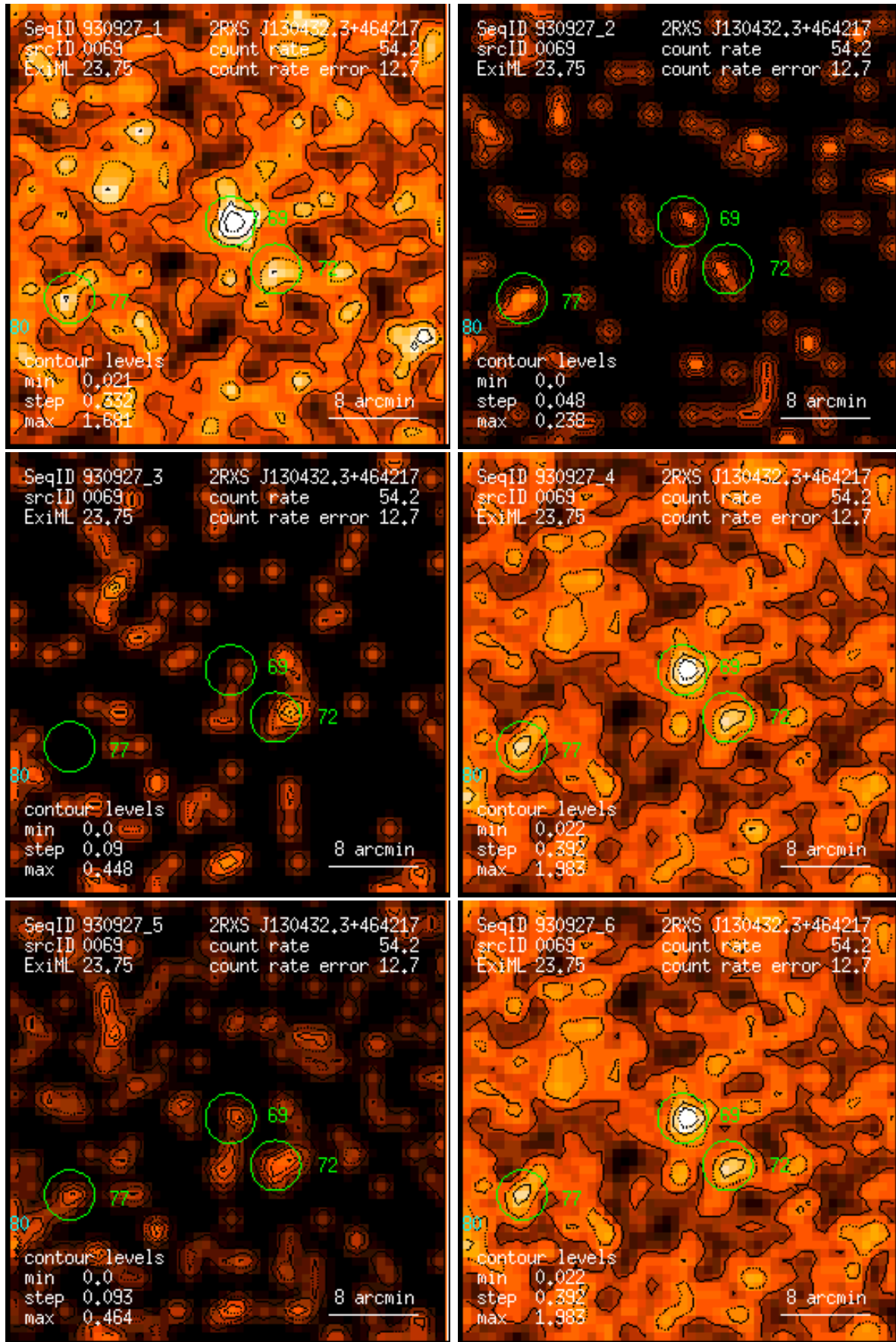
Figure 69: RASS 930927: detection 0069: band rate images, Gaussian filter: (1) PSPC channels 11 – 41, (2) 52 – 90, (3) 91 – 201, (4) 11 – 235, (5) 52 – 201, (6) 11 – 201. Broad band rates in counts/ks. Band rate contour levels in counts/ks/arcmin 2 .
