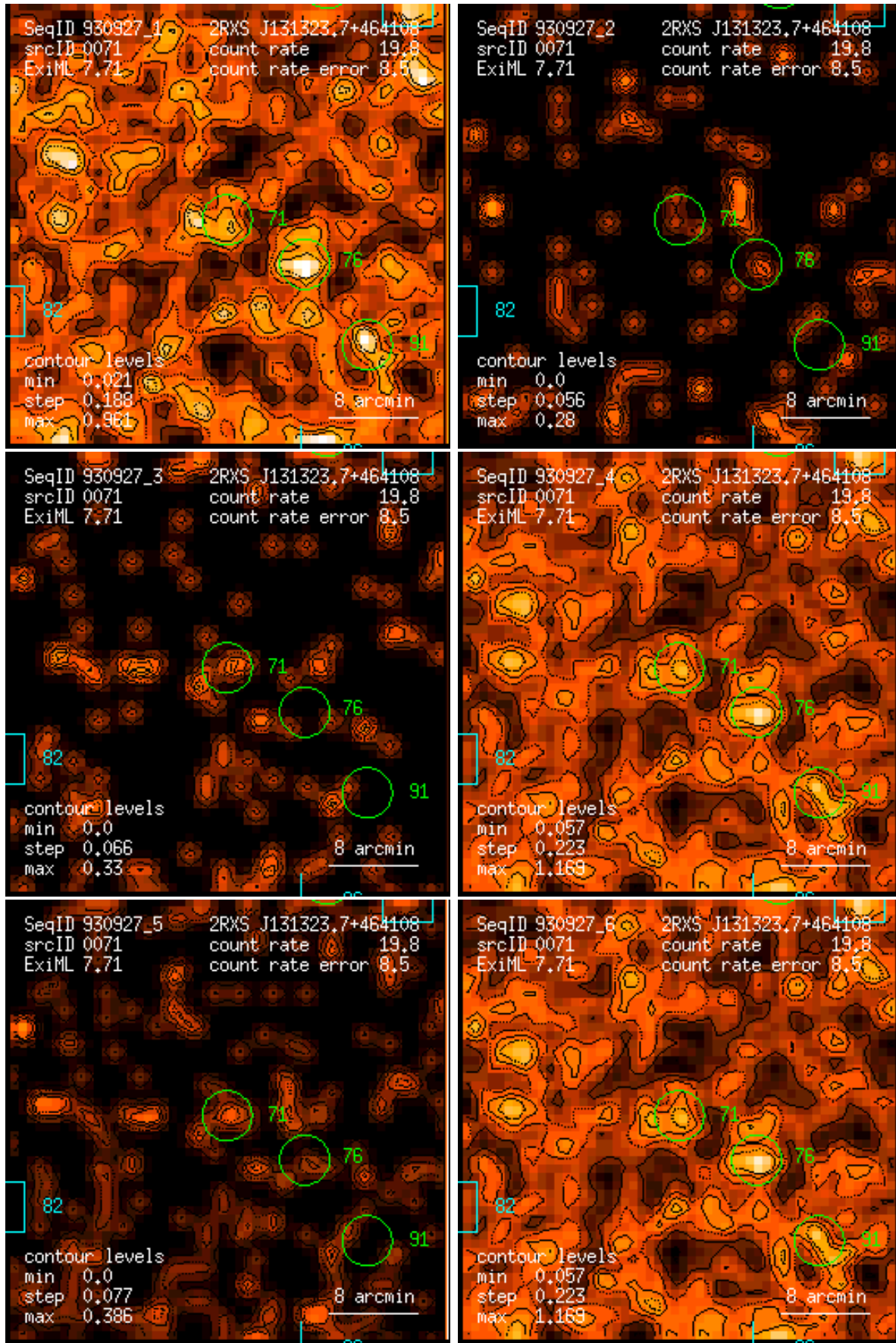
Figure 71: RASS 930927: detection 0071: band rate images, Gaussian filter: (1) PSPC channels 11 – 41, (2) 52 – 90, (3) 91 – 201, (4) 11 – 235, (5) 52 – 201, (6) 11 – 201. Broad band rates in counts/ks. Band rate contour levels in counts/ks/arcmin 2 .
