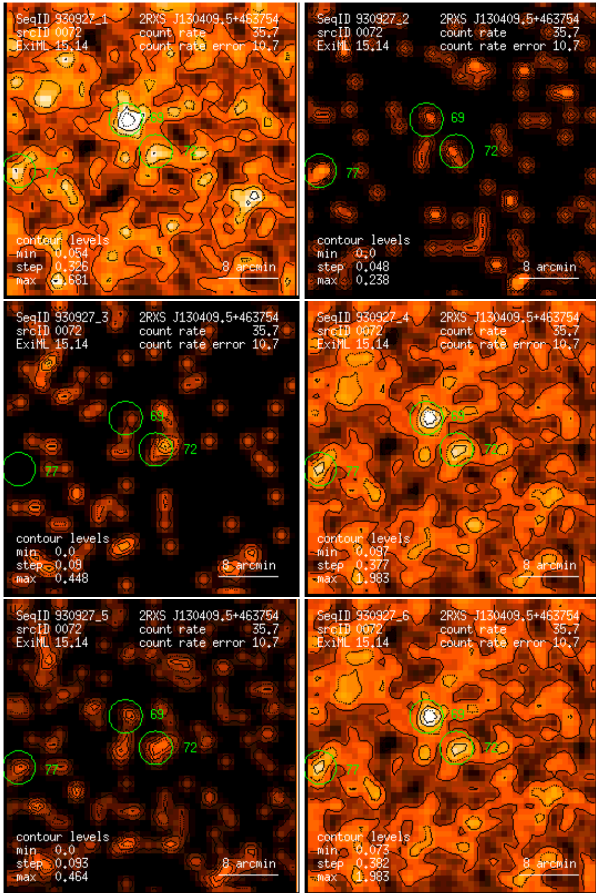
Figure 72: RASS 930927: detection 0072: band rate images, Gaussian filter: (1) PSPC channels 11 – 41, (2) 52 – 90, (3) 91 – 201, (4) 11 – 235, (5) 52 – 201, (6) 11 – 201. Broad band rates in counts/ks. Band rate contour levels in counts/ks/arcmin 2 .
