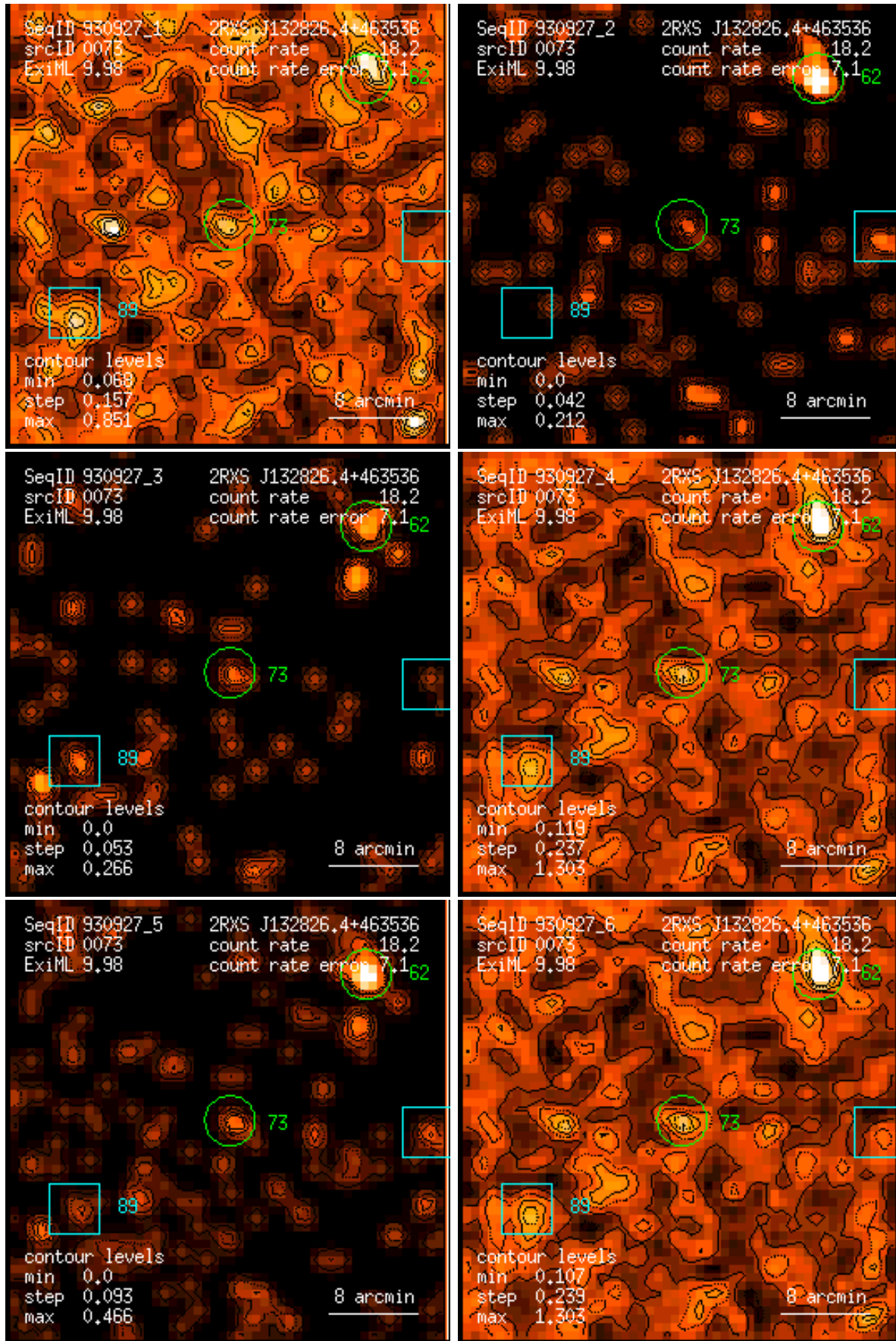
Figure 73: RASS 930927: detection 0073: band rate images, Gaussian filter: (1) PSPC channels 11 – 41, (2) 52 – 90, (3) 91 – 201, (4) 11 – 235, (5) 52 – 201, (6) 11 – 201. Broad band rates in counts/ks. Band rate contour levels in counts/ks/arcmin 2 .
