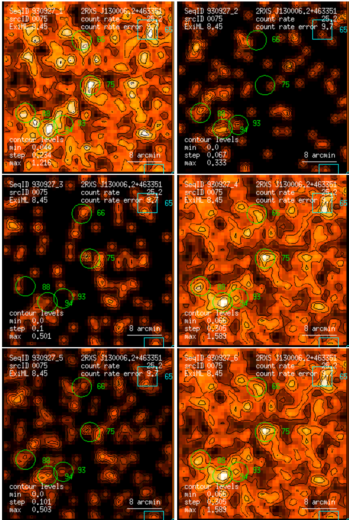
Figure 75: RASS 930927: detection 0075: band rate images, Gaussian filter: (1) PSPC channels 11 – 41, (2) 52 – 90, (3) 91 – 201, (4) 11 – 235, (5) 52 – 201, (6) 11 – 201. Broad band rates in counts/ks. Band rate contour levels in counts/ks/arcmin 2 .
