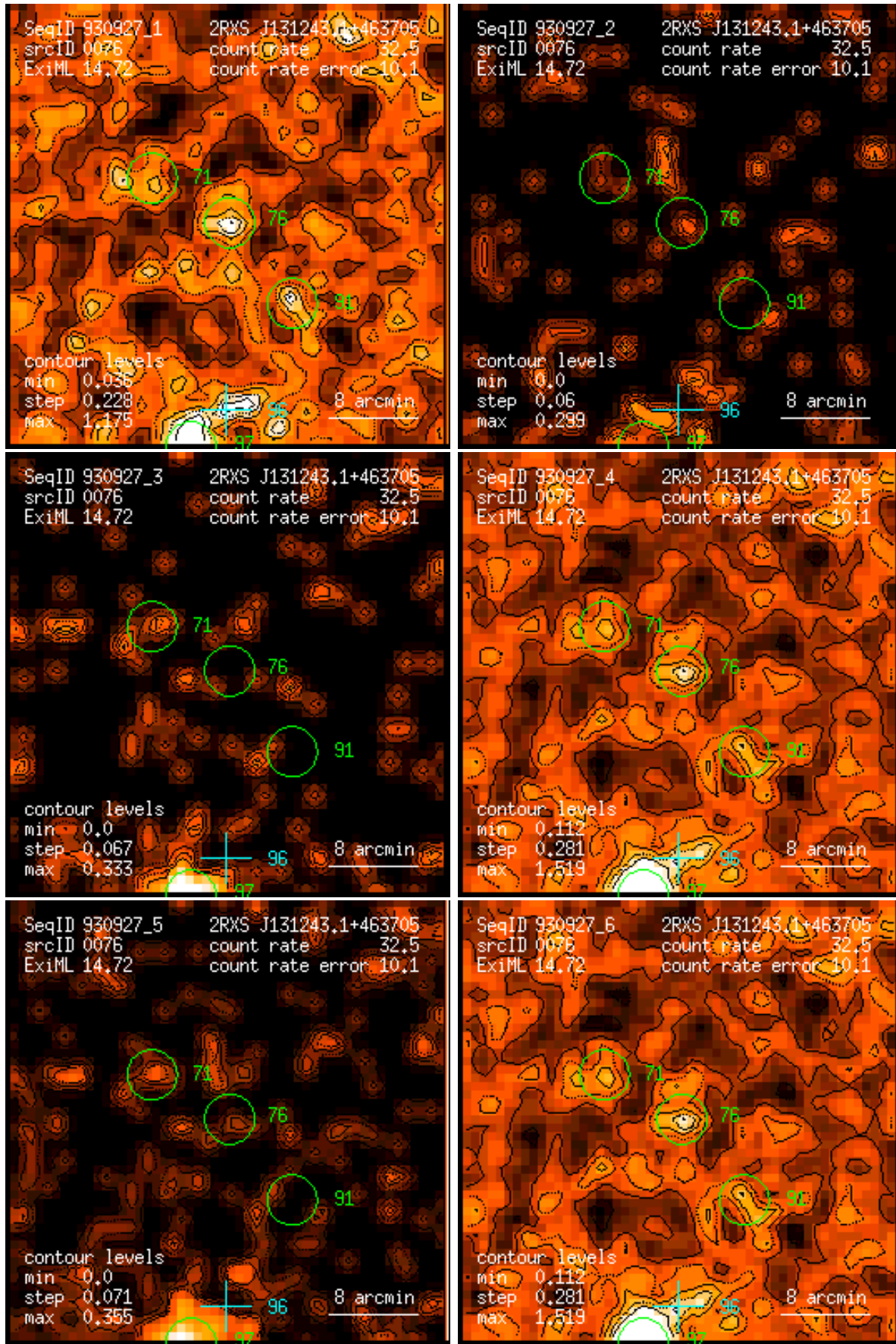
Figure 76: RASS 930927: detection 0076: band rate images, Gaussian filter: (1) PSPC channels 11 – 41, (2) 52 – 90, (3) 91 – 201, (4) 11 – 235, (5) 52 – 201, (6) 11 – 201. Broad band rates in counts/ks. Band rate contour levels in counts/ks/arcmin 2 .
