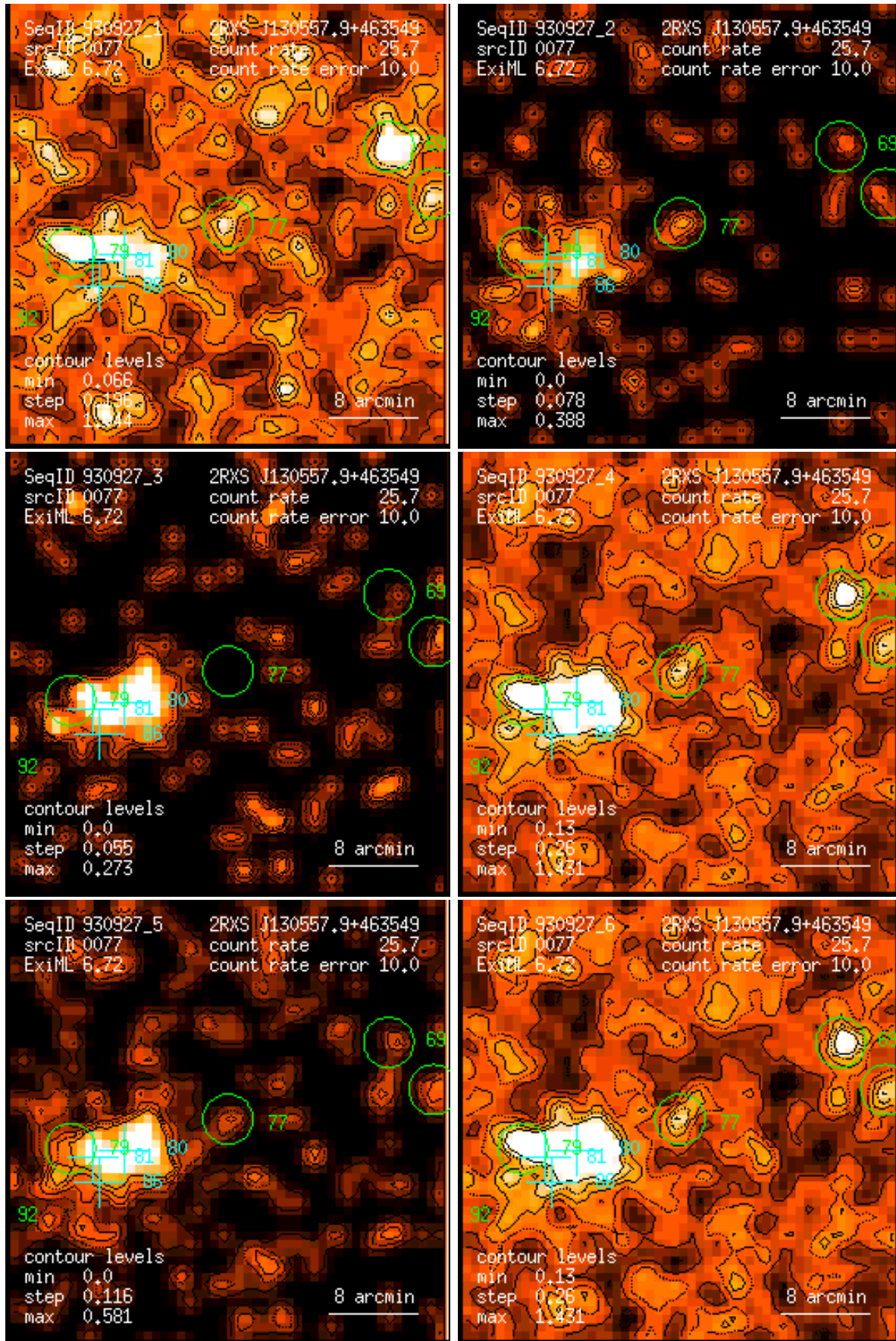
Figure 77: RASS 930927: detection 0077: band rate images, Gaussian filter: (1) PSPC channels 11 – 41, (2) 52 – 90, (3) 91 – 201, (4) 11 – 235, (5) 52 – 201, (6) 11 – 201. Broad band rates in counts/ks. Band rate contour levels in counts/ks/arcmin 2 .
