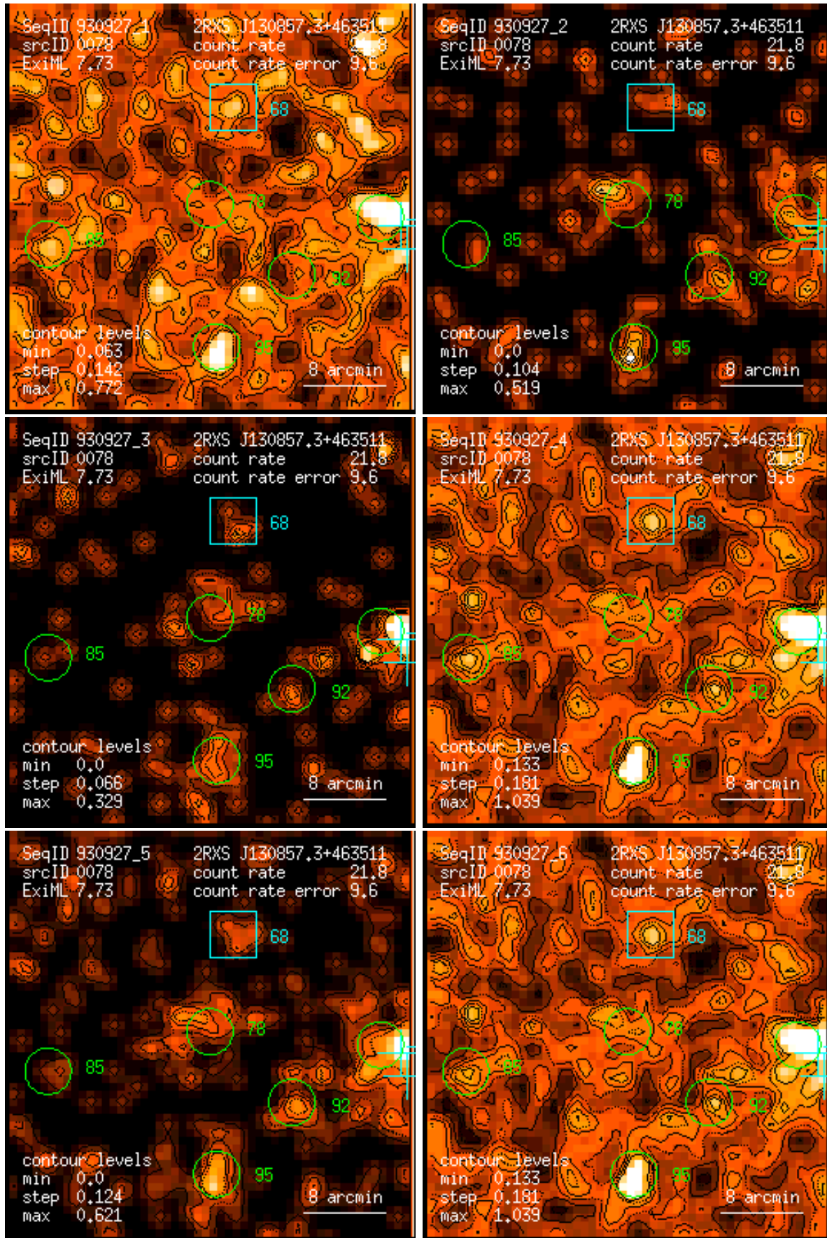
Figure 78: RASS 930927: detection 0078: band rate images, Gaussian filter: (1) PSPC channels 11 – 41, (2) 52 – 90, (3) 91 – 201, (4) 11 – 235, (5) 52 – 201, (6) 11 – 201. Broad band rates in counts/ks. Band rate contour levels in counts/ks/arcmin 2 .
