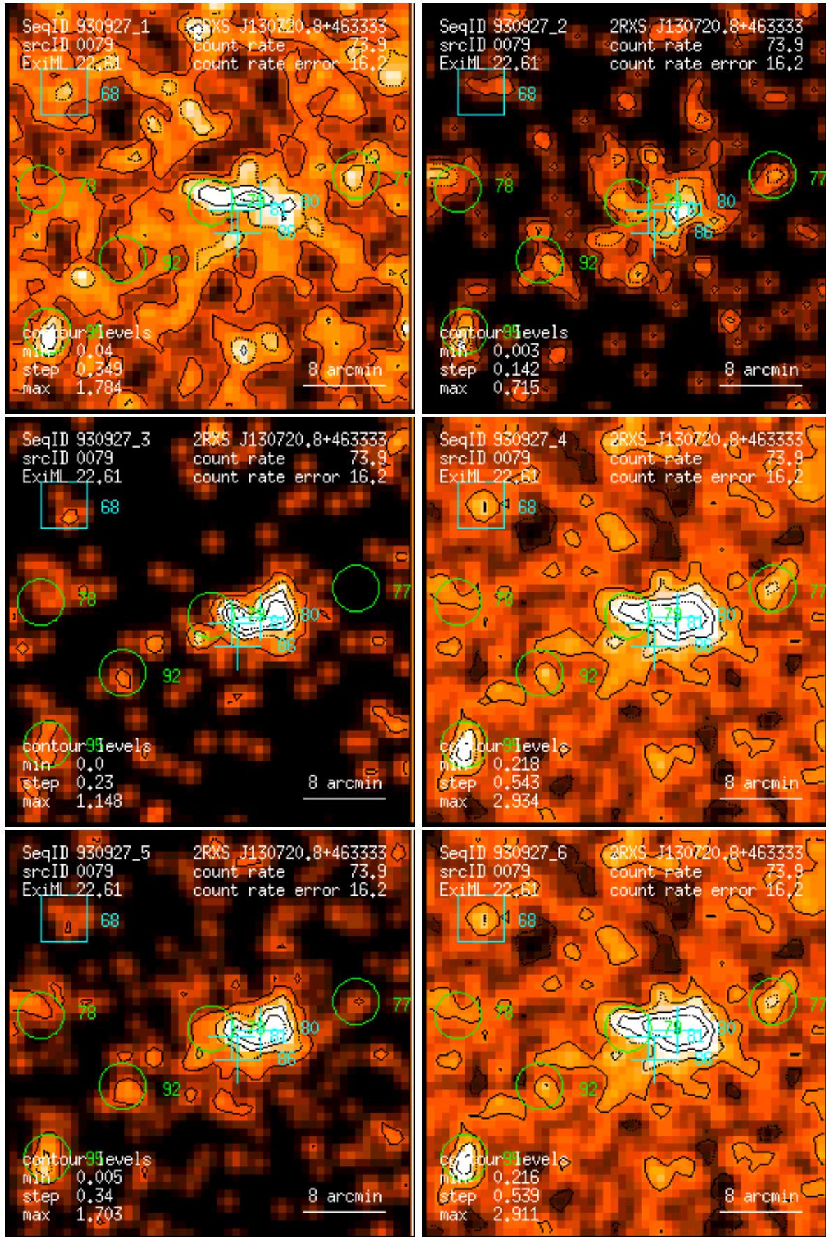
Figure 79: RASS 930927: detection 0079: band rate images, Gaussian filter: (1) PSPC channels 11 – 41, (2) 52 – 90, (3) 91 – 201, (4) 11 – 235, (5) 52 – 201, (6) 11 – 201. Broad band rates in counts/ks. Band rate contour levels in counts/ks/arcmin 2 .
