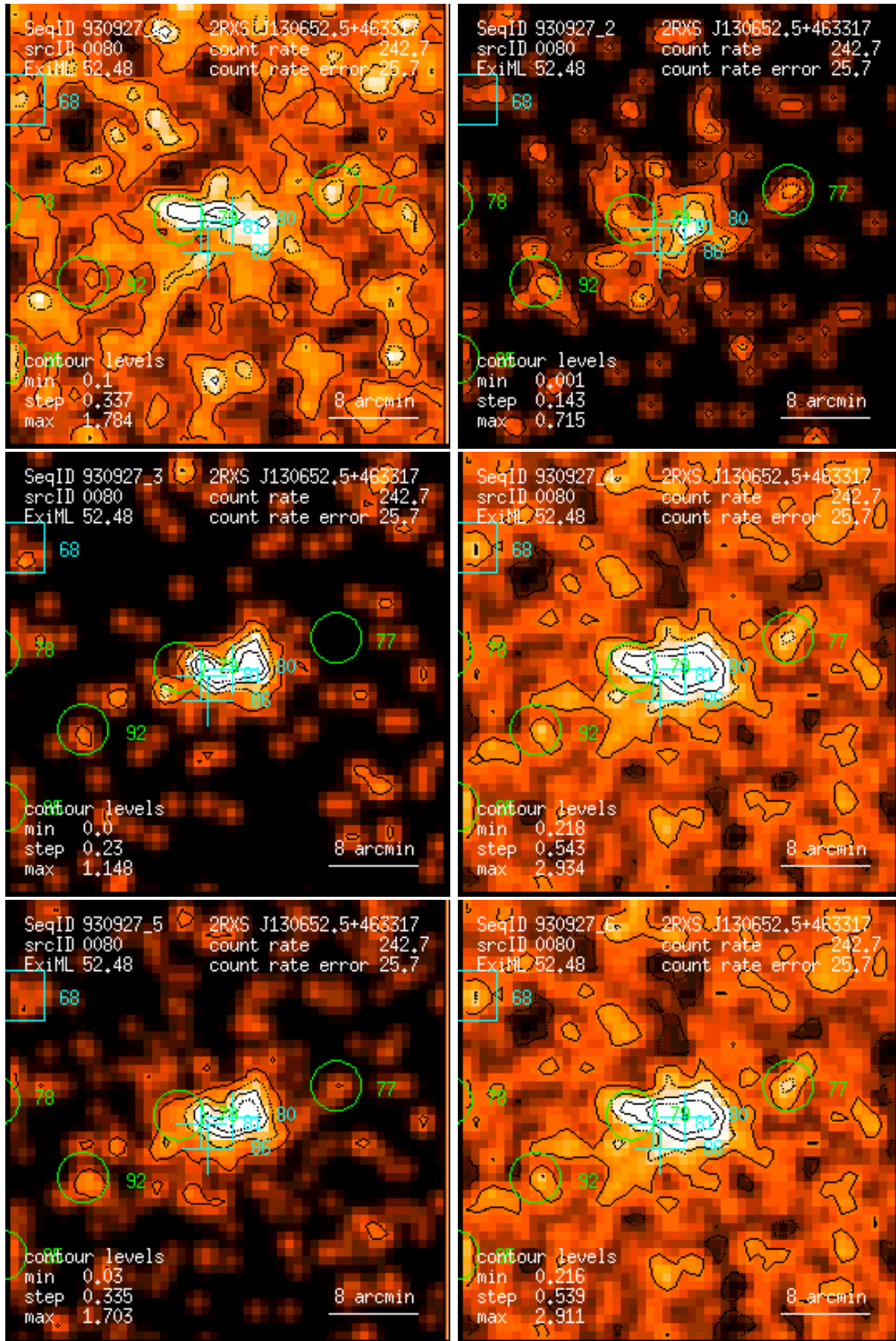
Figure 80: RASS 930927: detection 0080: band rate images, Gaussian filter: (1) PSPC channels 11 – 41, (2) 52 – 90, (3) 91 – 201, (4) 11 – 235, (5) 52 – 201, (6) 11 – 201. Broad band rates in counts/ks. Band rate contour levels in counts/ks/arcmin 2 .
