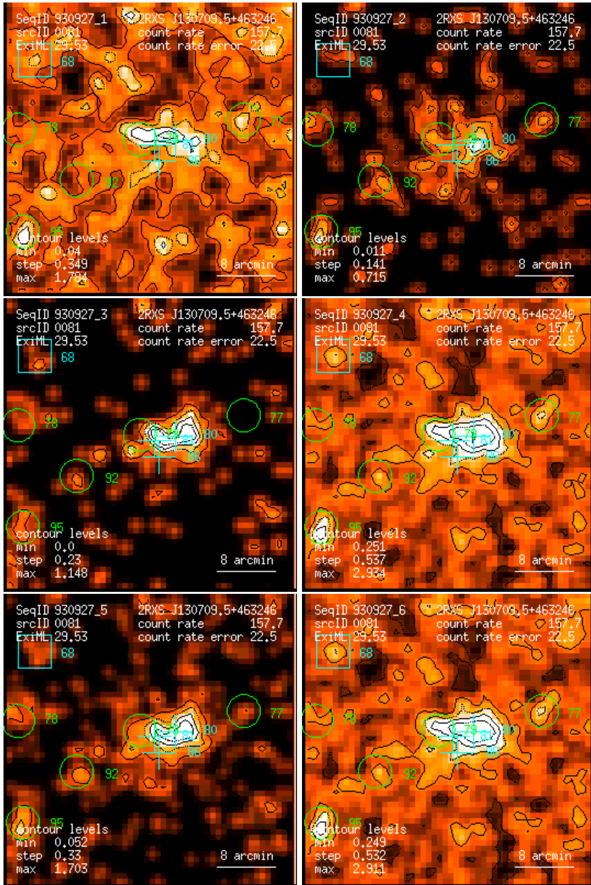
Figure 81: RASS 930927: detection 0081: band rate images, Gaussian filter: (1) PSPC channels 11 – 41, (2) 52 – 90, (3) 91 – 201, (4) 11 – 235, (5) 52 – 201, (6) 11 – 201. Broad band rates in counts/ks. Band rate contour levels in counts/ks/arcmin 2 .
