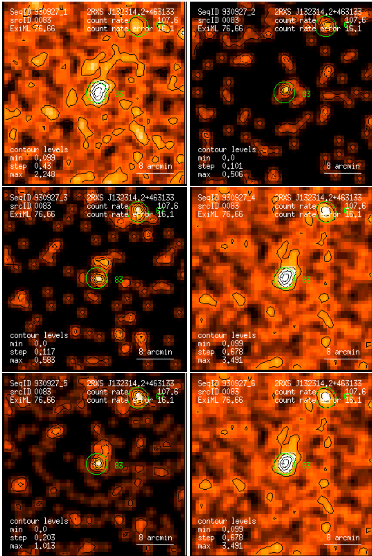
Figure 83: RASS 930927: detection 0083: band rate images, Gaussian filter: (1) PSPC channels 11 – 41, (2) 52 – 90, (3) 91 – 201, (4) 11 – 235, (5) 52 – 201, (6) 11 – 201. Broad band rates in counts/ks. Band rate contour levels in counts/ks/arcmin 2 .
