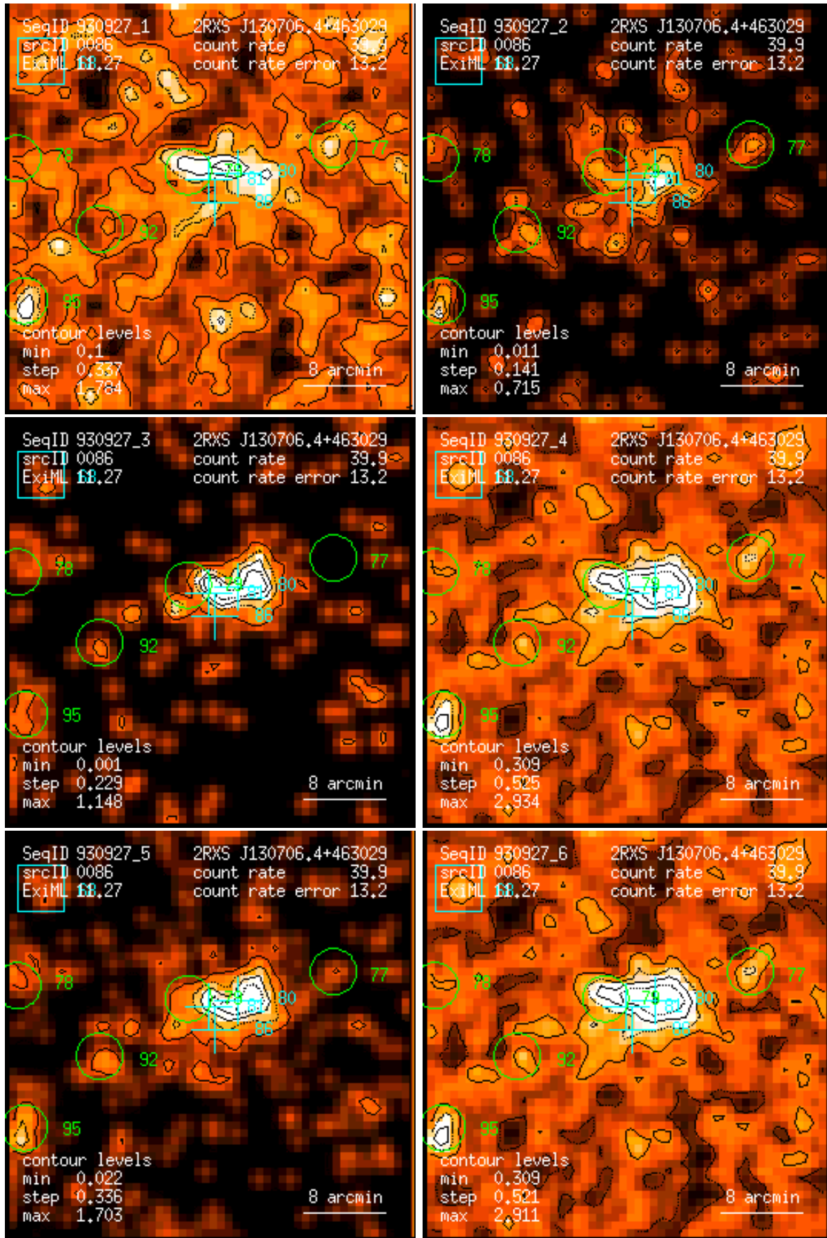
Figure 86: RASS 930927: detection 0086: band rate images, Gaussian filter: (1) PSPC channels 11 – 41, (2) 52 – 90, (3) 91 – 201, (4) 11 – 235, (5) 52 – 201, (6) 11 – 201. Broad band rates in counts/ks. Band rate contour levels in counts/ks/arcmin 2 .
