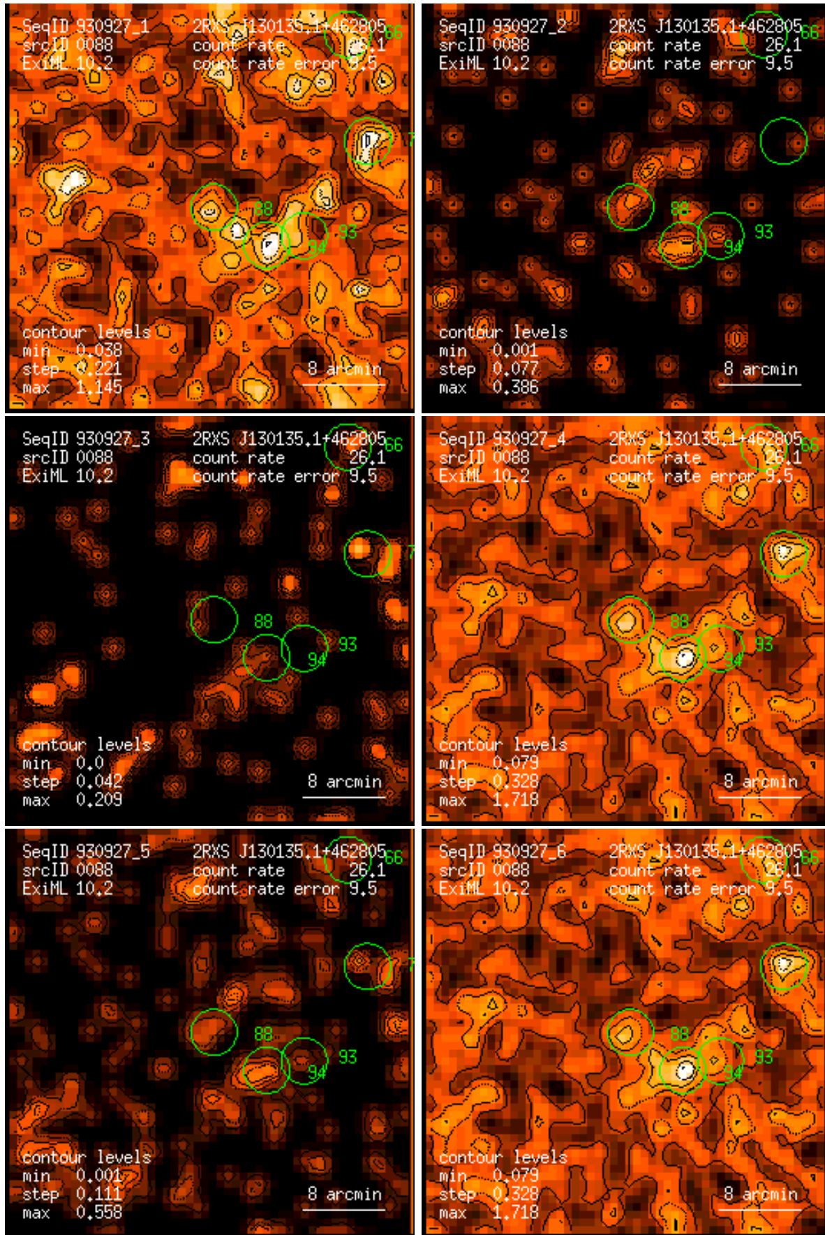
Figure 88: RASS 930927: detection 0088: band rate images, Gaussian filter: (1) PSPC channels 11 – 41, (2) 52 – 90, (3) 91 – 201, (4) 11 – 235, (5) 52 – 201, (6) 11 – 201. Broad band rates in counts/ks. Band rate contour levels in counts/ks/arcmin 2 .
