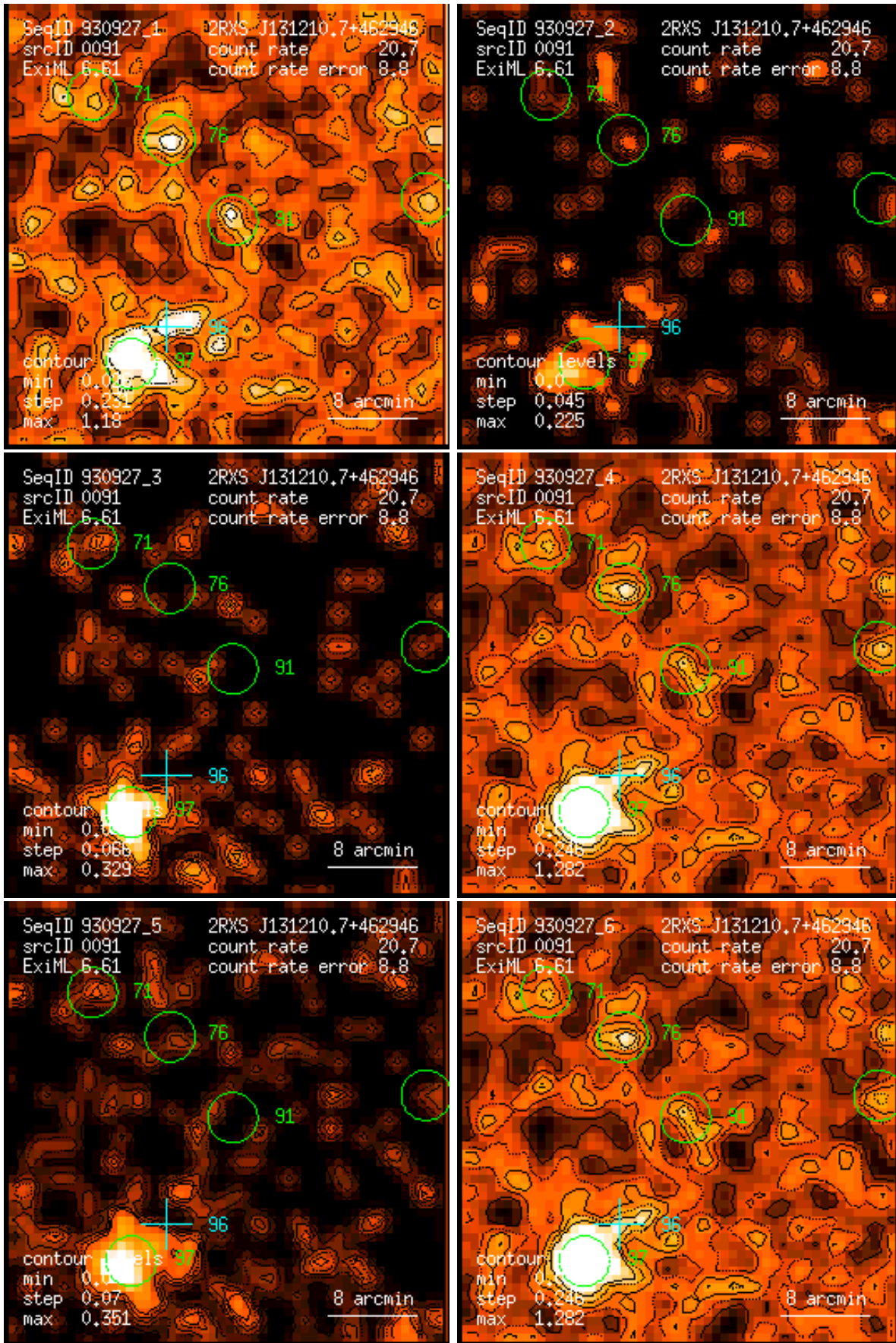
Figure 91: RASS 930927: detection 0091: band rate images, Gaussian filter: (1) PSPC channels 11 – 41, (2) 52 – 90, (3) 91 – 201, (4) 11 – 235, (5) 52 – 201, (6) 11 – 201. Broad band rates in counts/ks. Band rate contour levels in counts/ks/arcmin 2 .
