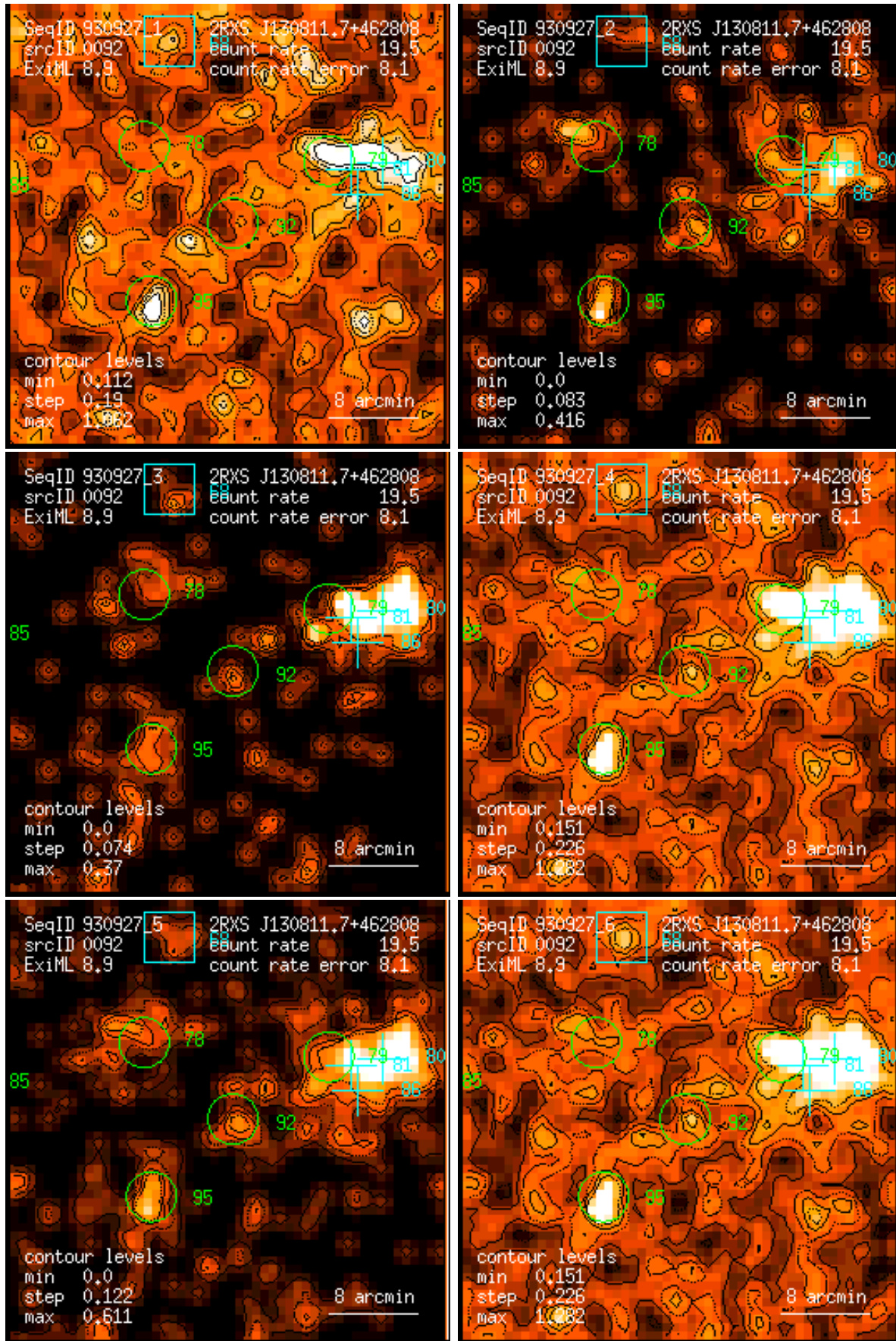
Figure 92: RASS 930927: detection 0092: band rate images, Gaussian filter: (1) PSPC channels 11 – 41, (2) 52 – 90, (3) 91 – 201, (4) 11 – 235, (5) 52 – 201, (6) 11 – 201. Broad band rates in counts/ks. Band rate contour levels in counts/ks/arcmin 2 .
