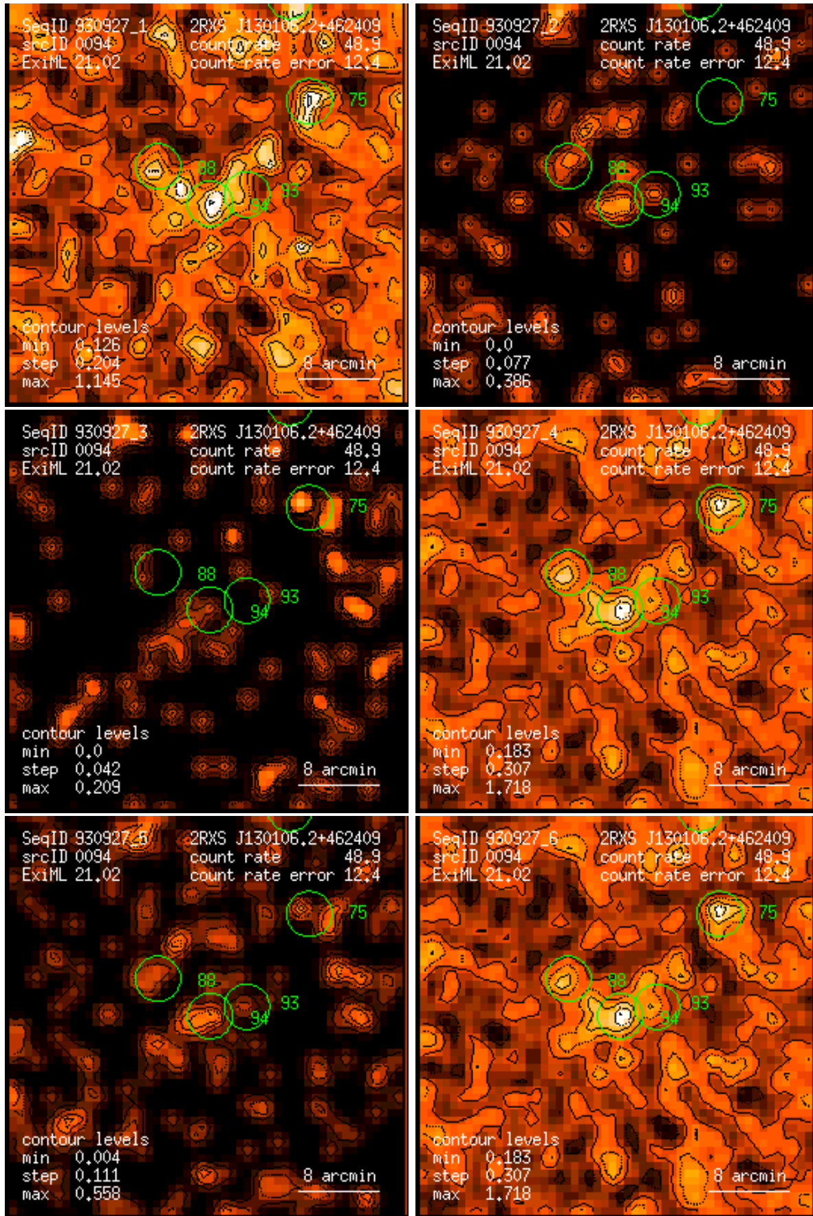
Figure 94: RASS 930927: detection 0094: band rate images, Gaussian filter: (1) PSPC channels 11 – 41, (2) 52 – 90, (3) 91 – 201, (4) 11 – 235, (5) 52 – 201, (6) 11 – 201. Broad band rates in counts/ks. Band rate contour levels in counts/ks/arcmin 2 .
