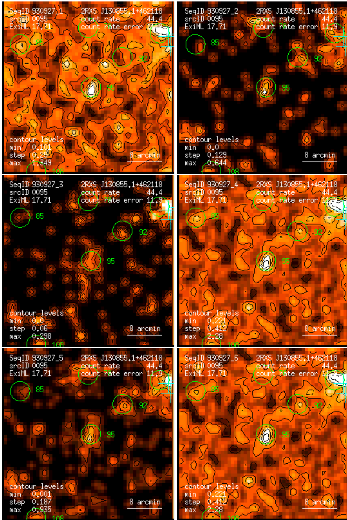
Figure 95: RASS 930927: detection 0095: band rate images, Gaussian filter: (1) PSPC channels 11 – 41, (2) 52 – 90, (3) 91 – 201, (4) 11 – 235, (5) 52 – 201, (6) 11 – 201. Broad band rates in counts/ks. Band rate contour levels in counts/ks/arcmin 2 .
