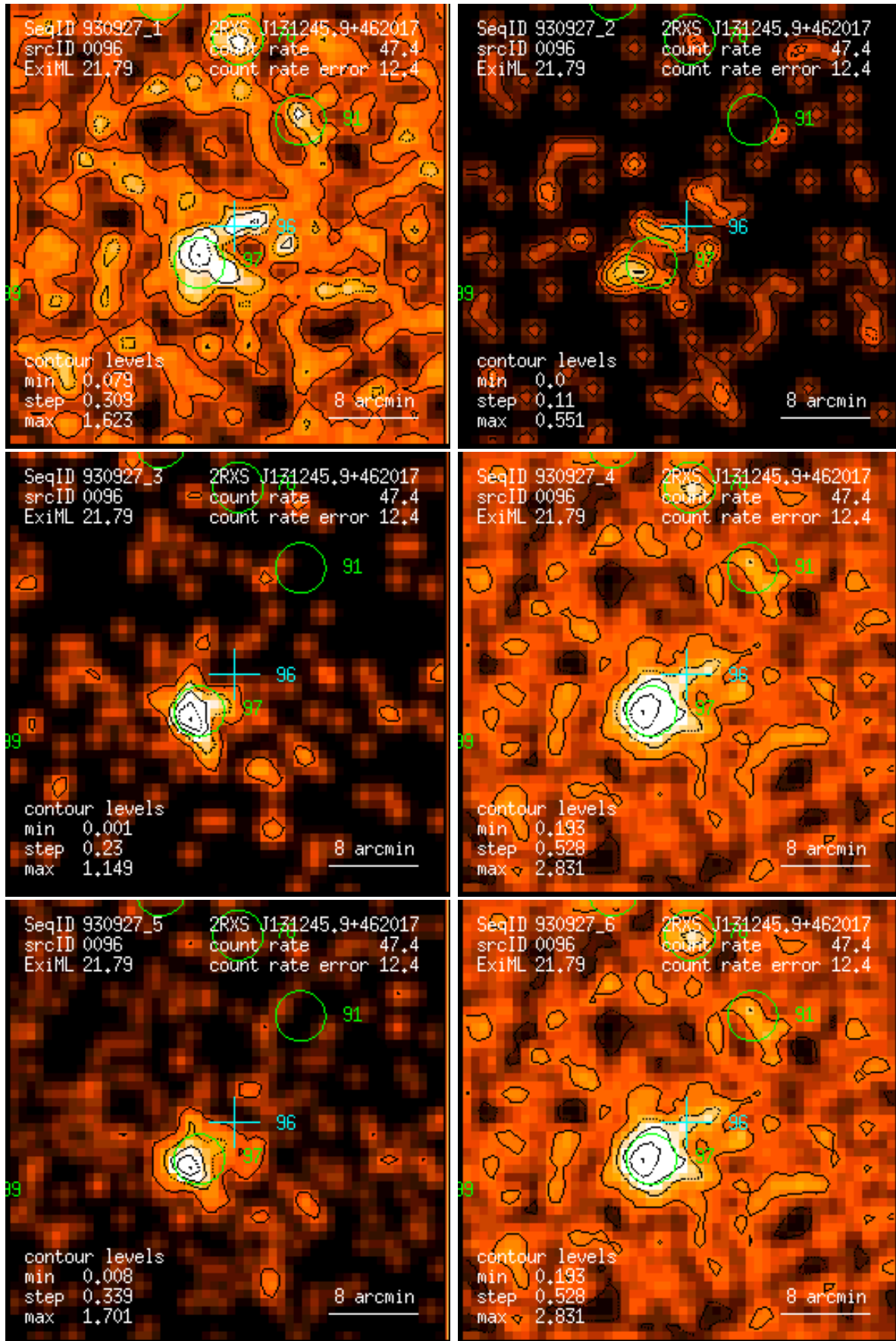
Figure 96: RASS 930927: detection 0096: band rate images, Gaussian filter: (1) PSPC channels 11 – 41, (2) 52 – 90, (3) 91 – 201, (4) 11 – 235, (5) 52 – 201, (6) 11 – 201. Broad band rates in counts/ks. Band rate contour levels in counts/ks/arcmin 2 .
