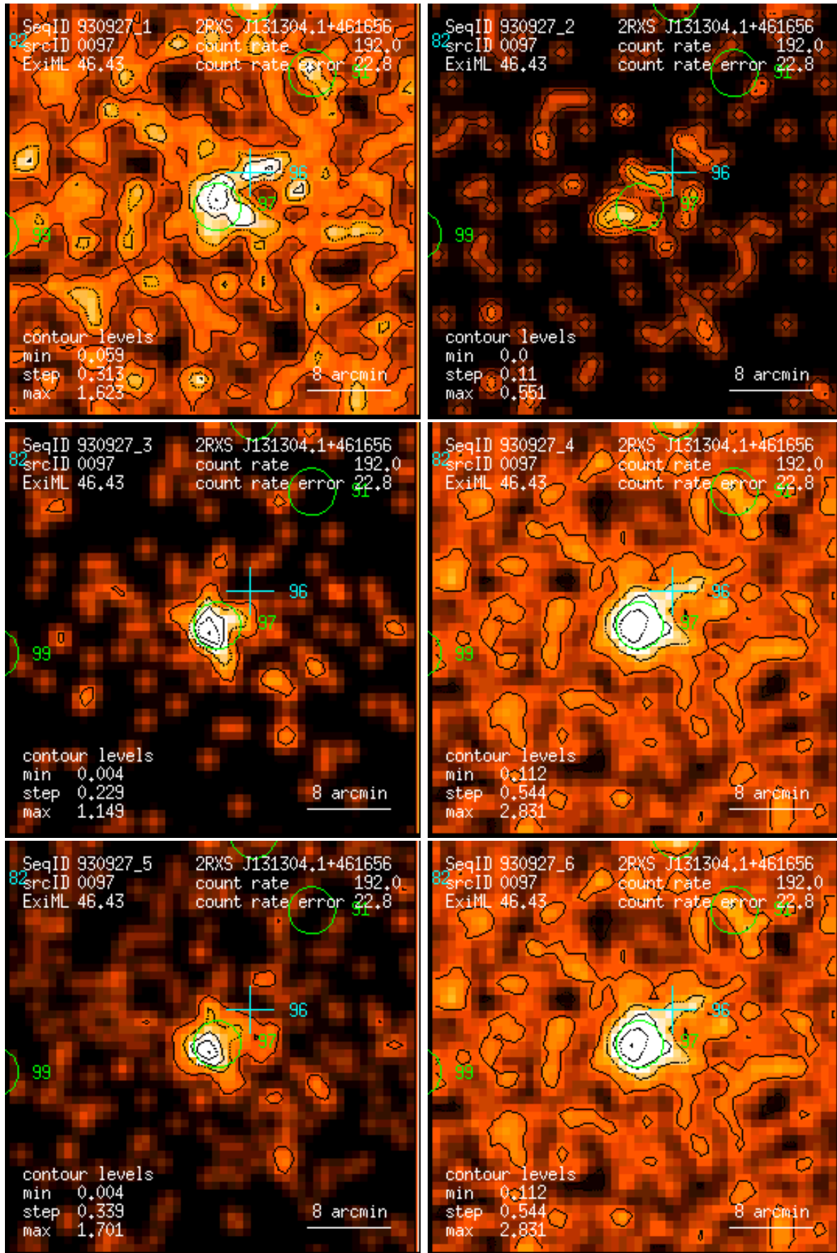
Figure 97: RASS 930927: detection 0097: band rate images, Gaussian filter: (1) PSPC channels 11 – 41, (2) 52 – 90, (3) 91 – 201, (4) 11 – 235, (5) 52 – 201, (6) 11 – 201. Broad band rates in counts/ks. Band rate contour levels in counts/ks/arcmin 2 .
