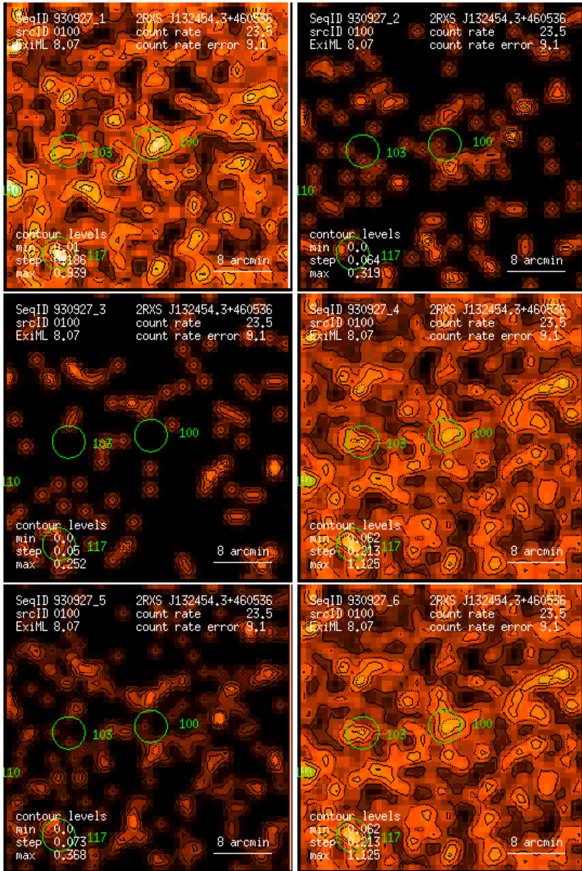
Figure 100: RASS 930927: detection 0100: band rate images, Gaussian filter: (1) PSPC channels 11 – 41, (2) 52 – 90, (3) 91 – 201, (4) 11 – 235, (5) 52 – 201, (6) 11 – 201. Broad band rates in counts/ks. Band rate contour levels in counts/ks/arcmin 2 .
