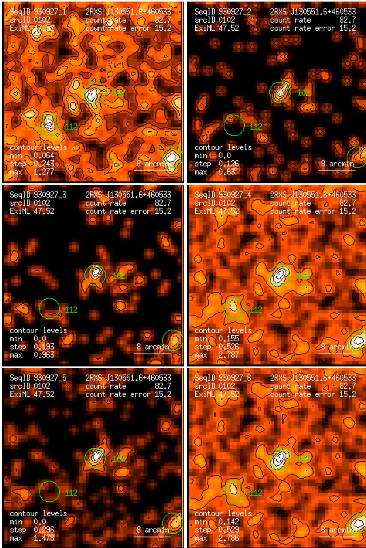
Figure 102: RASS 930927: detection 0102: band rate images, Gaussian filter: (1) PSPC channels 11 – 41, (2) 52 – 90, (3) 91 – 201, (4) 11 – 235, (5) 52 – 201, (6) 11 – 201. Broad band rates in counts/ks. Band rate contour levels in counts/ks/arcmin 2 .
