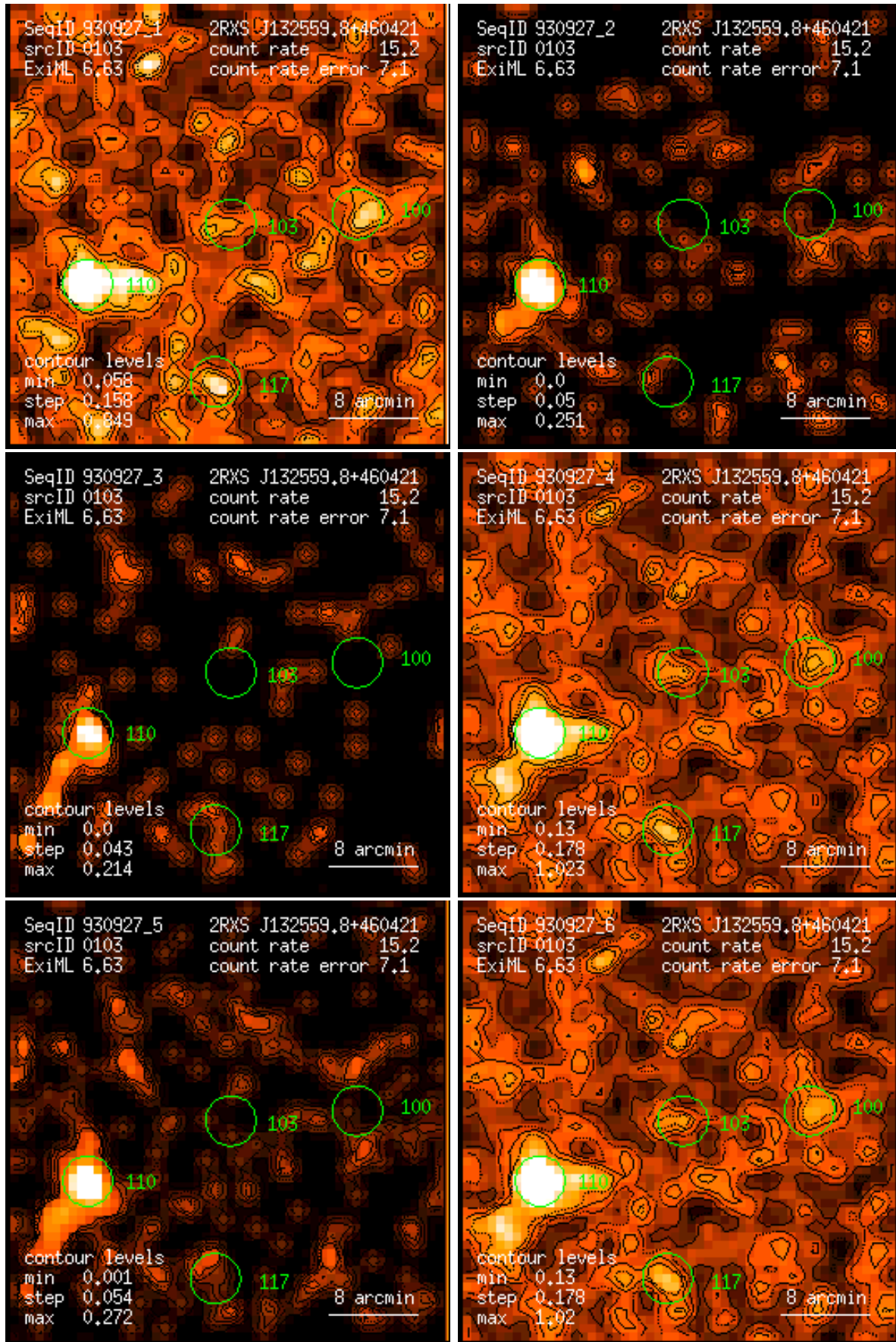
Figure 103: RASS 930927: detection 0103: band rate images, Gaussian filter: (1) PSPC channels 11 – 41, (2) 52 – 90, (3) 91 – 201, (4) 11 – 235, (5) 52 – 201, (6) 11 – 201. Broad band rates in counts/ks. Band rate contour levels in counts/ks/arcmin 2 .
