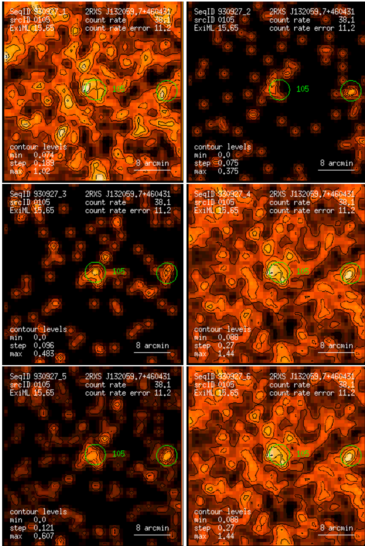
Figure 105: RASS 930927: detection 0105: band rate images, Gaussian filter: (1) PSPC channels 11 – 41, (2) 52 – 90, (3) 91 – 201, (4) 11 – 235, (5) 52 – 201, (6) 11 – 201. Broad band rates in counts/ks. Band rate contour levels in counts/ks/arcmin 2 .
