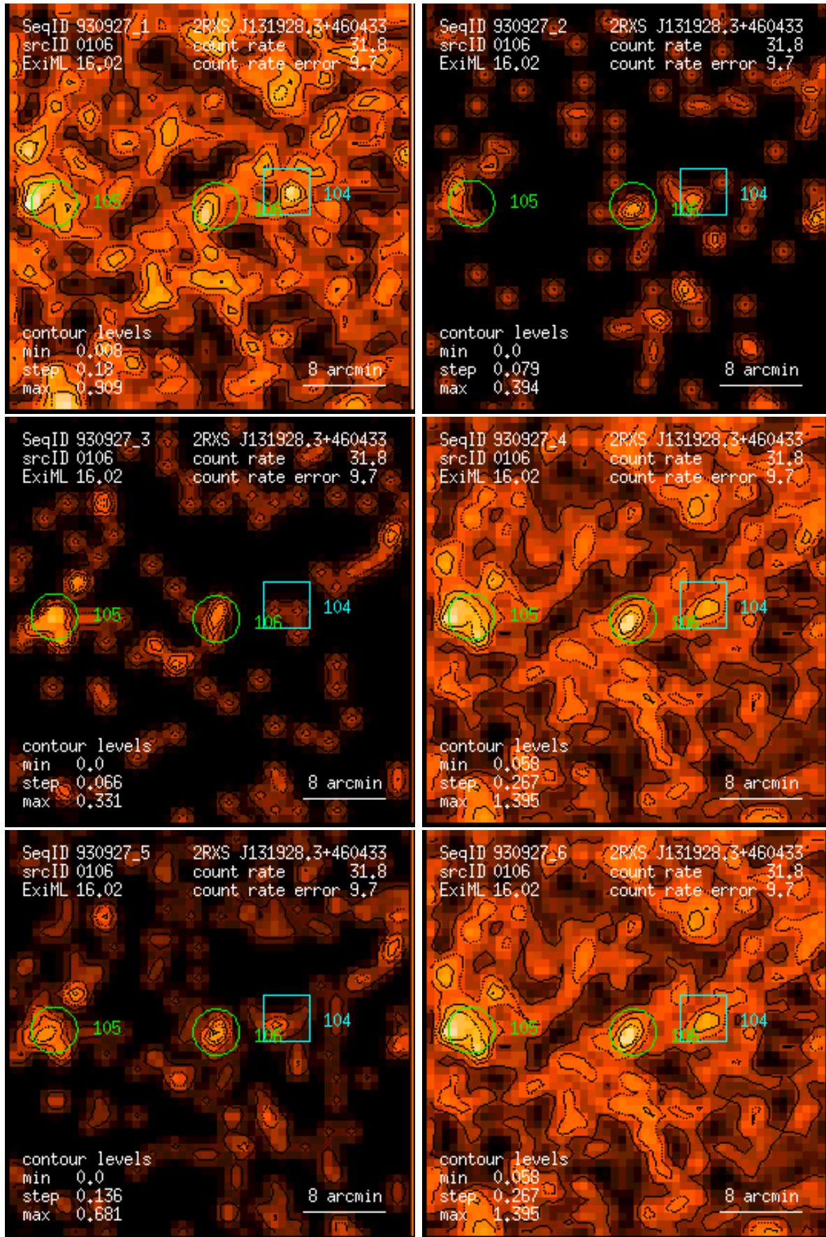
Figure 106: RASS 930927: detection 0106: band rate images, Gaussian filter: (1) PSPC channels 11 – 41, (2) 52 – 90, (3) 91 – 201, (4) 11 – 235, (5) 52 – 201, (6) 11 – 201. Broad band rates in counts/ks. Band rate contour levels in counts/ks/arcmin 2 .
