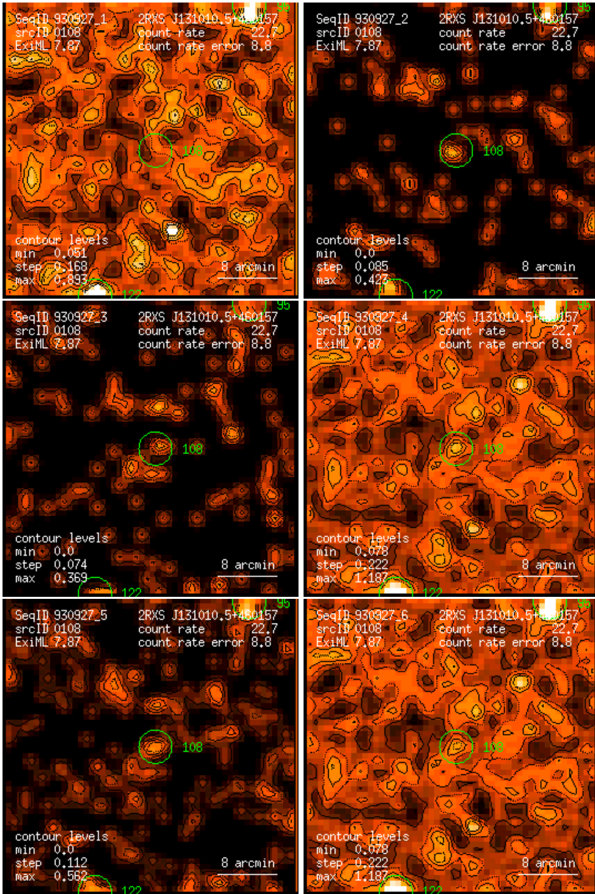
Figure 108: RASS 930927: detection 0108: band rate images, Gaussian filter: (1) PSPC channels 11 – 41, (2) 52 – 90, (3) 91 – 201, (4) 11 – 235, (5) 52 – 201, (6) 11 – 201. Broad band rates in counts/ks. Band rate contour levels in counts/ks/arcmin 2 .
