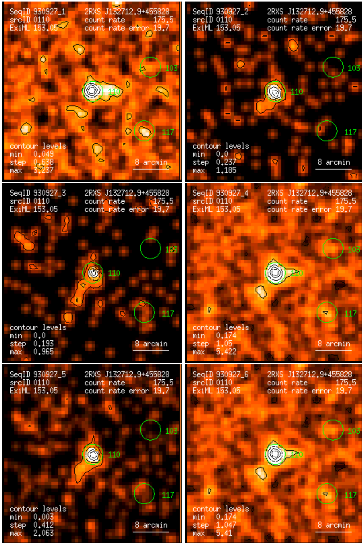
Figure 110: RASS 930927: detection 0110: band rate images, Gaussian filter: (1) PSPC channels 11 – 41, (2) 52 – 90, (3) 91 – 201, (4) 11 – 235, (5) 52 – 201, (6) 11 – 201. Broad band rates in counts/ks. Band rate contour levels in counts/ks/arcmin 2 .
