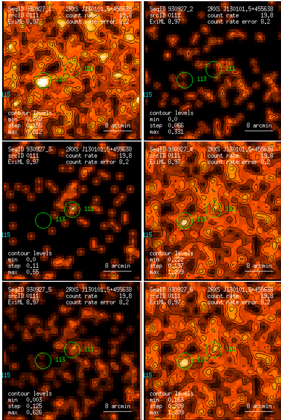
Figure 111: RASS 930927: detection 0111: band rate images, Gaussian filter: (1) PSPC channels 11 – 41, (2) 52 – 90, (3) 91 – 201, (4) 11 – 235, (5) 52 – 201, (6) 11 – 201. Broad band rates in counts/ks. Band rate contour levels in counts/ks/arcmin 2 .
