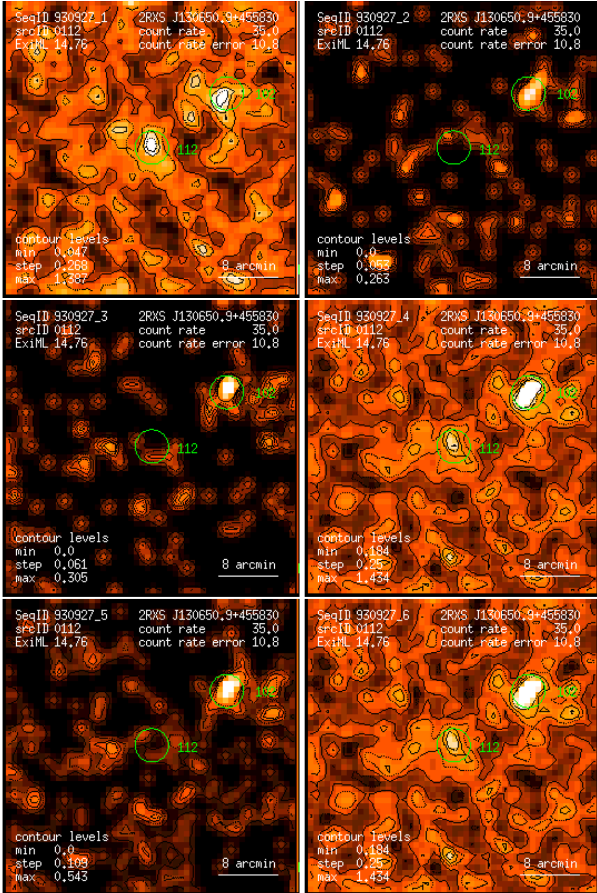
Figure 112: RASS 930927: detection 0112: band rate images, Gaussian filter: (1) PSPC channels 11 – 41, (2) 52 – 90, (3) 91 – 201, (4) 11 – 235, (5) 52 – 201, (6) 11 – 201. Broad band rates in counts/ks. Band rate contour levels in counts/ks/arcmin 2 .
