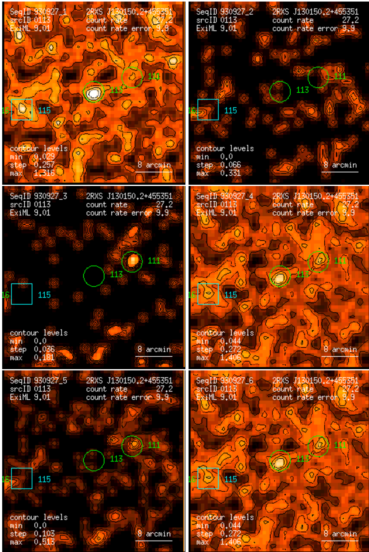
Figure 113: RASS 930927: detection 0113: band rate images, Gaussian filter: (1) PSPC channels 11 – 41, (2) 52 – 90, (3) 91 – 201, (4) 11 – 235, (5) 52 – 201, (6) 11 – 201. Broad band rates in counts/ks. Band rate contour levels in counts/ks/arcmin 2 .
