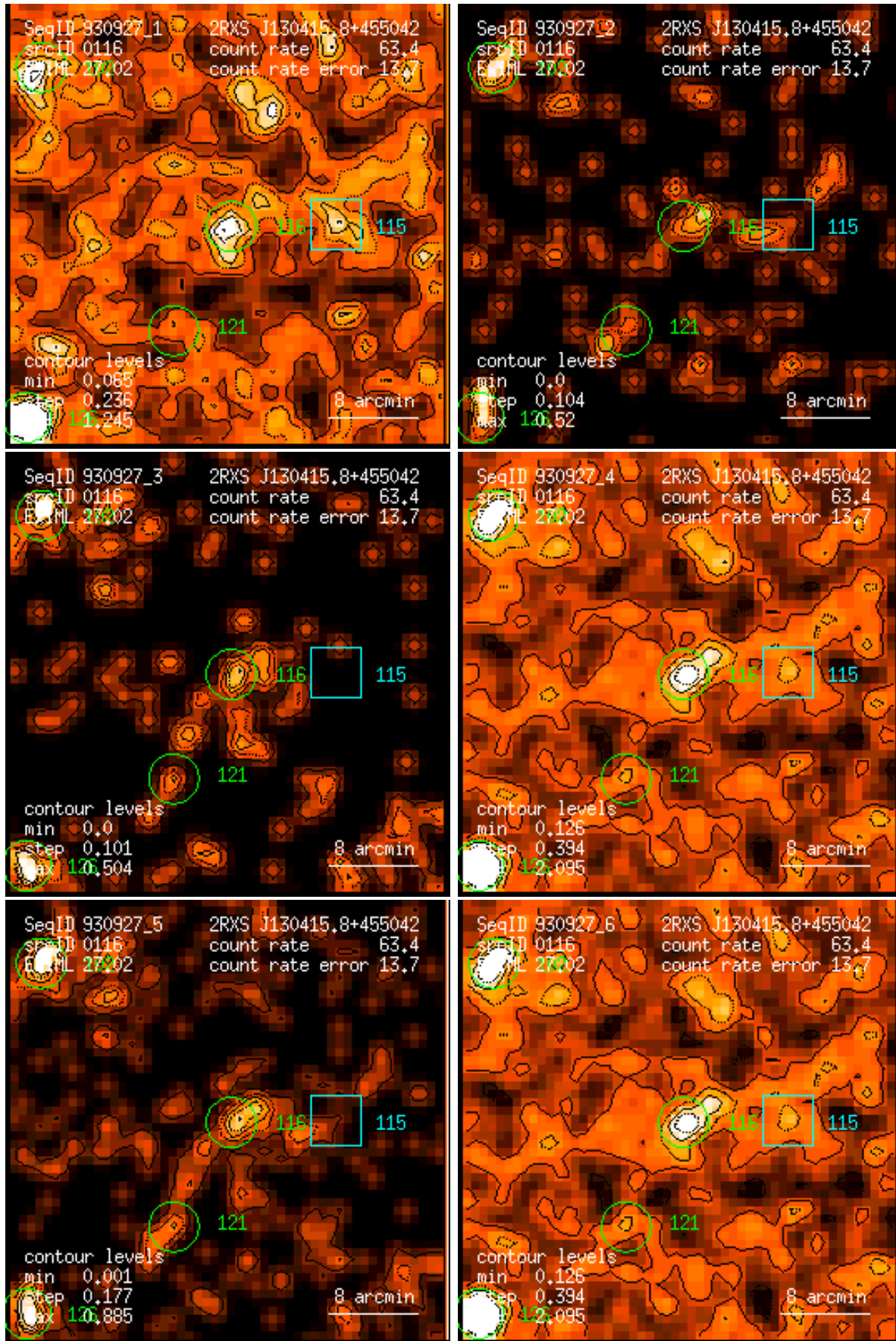
Figure 116: RASS 930927: detection 0116: band rate images, Gaussian filter: (1) PSPC channels 11 – 41, (2) 52 – 90, (3) 91 – 201, (4) 11 – 235, (5) 52 – 201, (6) 11 – 201. Broad band rates in counts/ks. Band rate contour levels in counts/ks/arcmin 2 .
