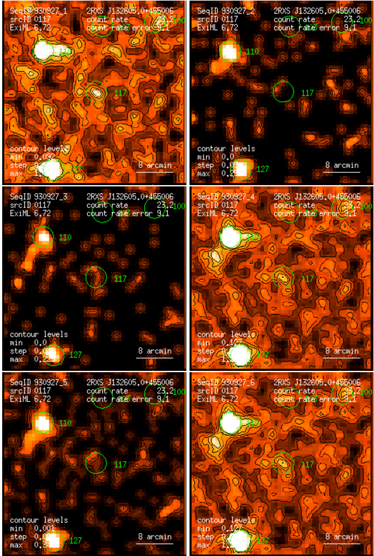
Figure 117: RASS 930927: detection 0117: band rate images, Gaussian filter: (1) PSPC channels 11 – 41, (2) 52 – 90, (3) 91 – 201, (4) 11 – 235, (5) 52 – 201, (6) 11 – 201. Broad band rates in counts/ks. Band rate contour levels in counts/ks/arcmin 2 .
