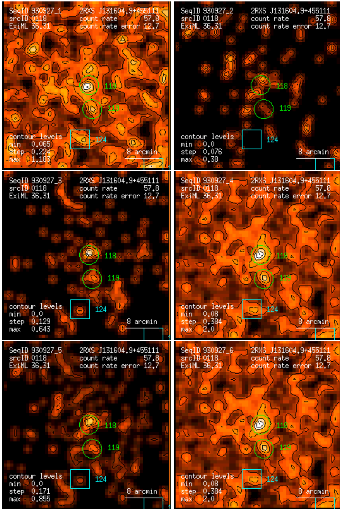
Figure 118: RASS 930927: detection 0118: band rate images, Gaussian filter: (1) PSPC channels 11 – 41, (2) 52 – 90, (3) 91 – 201, (4) 11 – 235, (5) 52 – 201, (6) 11 – 201. Broad band rates in counts/ks. Band rate contour levels in counts/ks/arcmin 2 .
