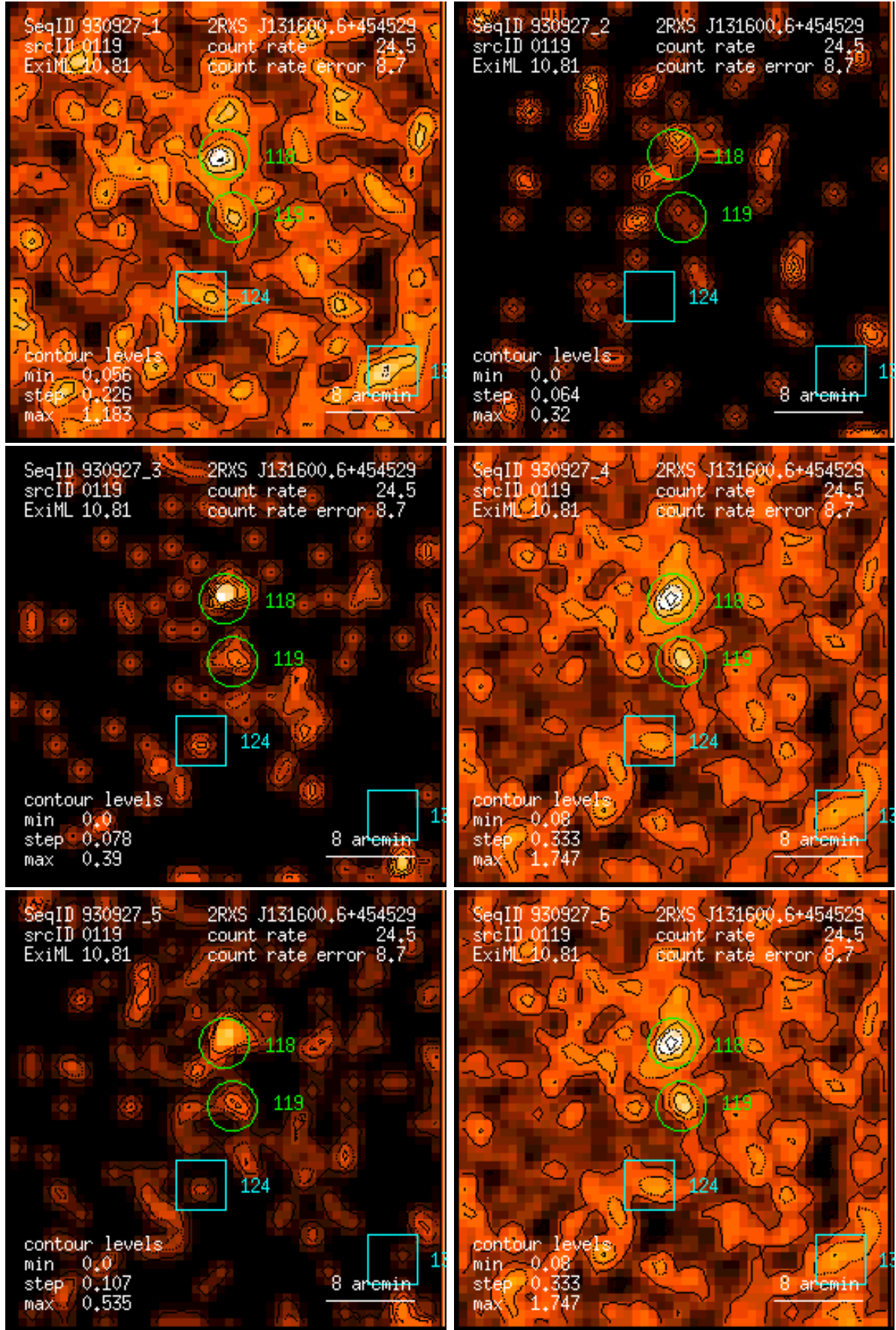
Figure 119: RASS 930927: detection 0119: band rate images, Gaussian filter: (1) PSPC channels 11 – 41, (2) 52 – 90, (3) 91 – 201, (4) 11 – 235, (5) 52 – 201, (6) 11 – 201. Broad band rates in counts/ks. Band rate contour levels in counts/ks/arcmin 2 .
