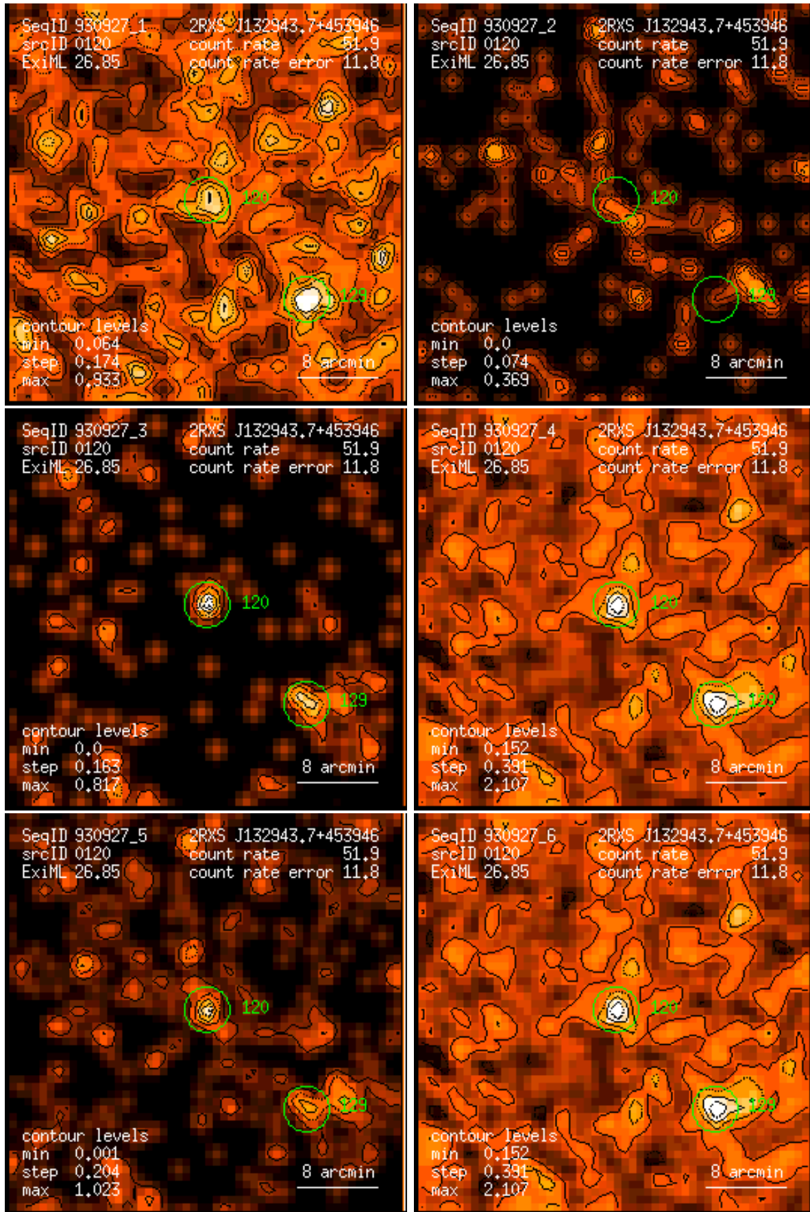
Figure 120: RASS 930927: detection 0120: band rate images, Gaussian filter: (1) PSPC channels 11 – 41, (2) 52 – 90, (3) 91 – 201, (4) 11 – 235, (5) 52 – 201, (6) 11 – 201. Broad band rates in counts/ks. Band rate contour levels in counts/ks/arcmin 2 .
