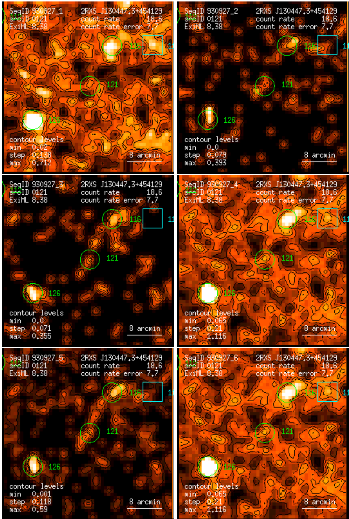
Figure 121: RASS 930927: detection 0121: band rate images, Gaussian filter: (1) PSPC channels 11 – 41, (2) 52 – 90, (3) 91 – 201, (4) 11 – 235, (5) 52 – 201, (6) 11 – 201. Broad band rates in counts/ks. Band rate contour levels in counts/ks/arcmin 2 .
