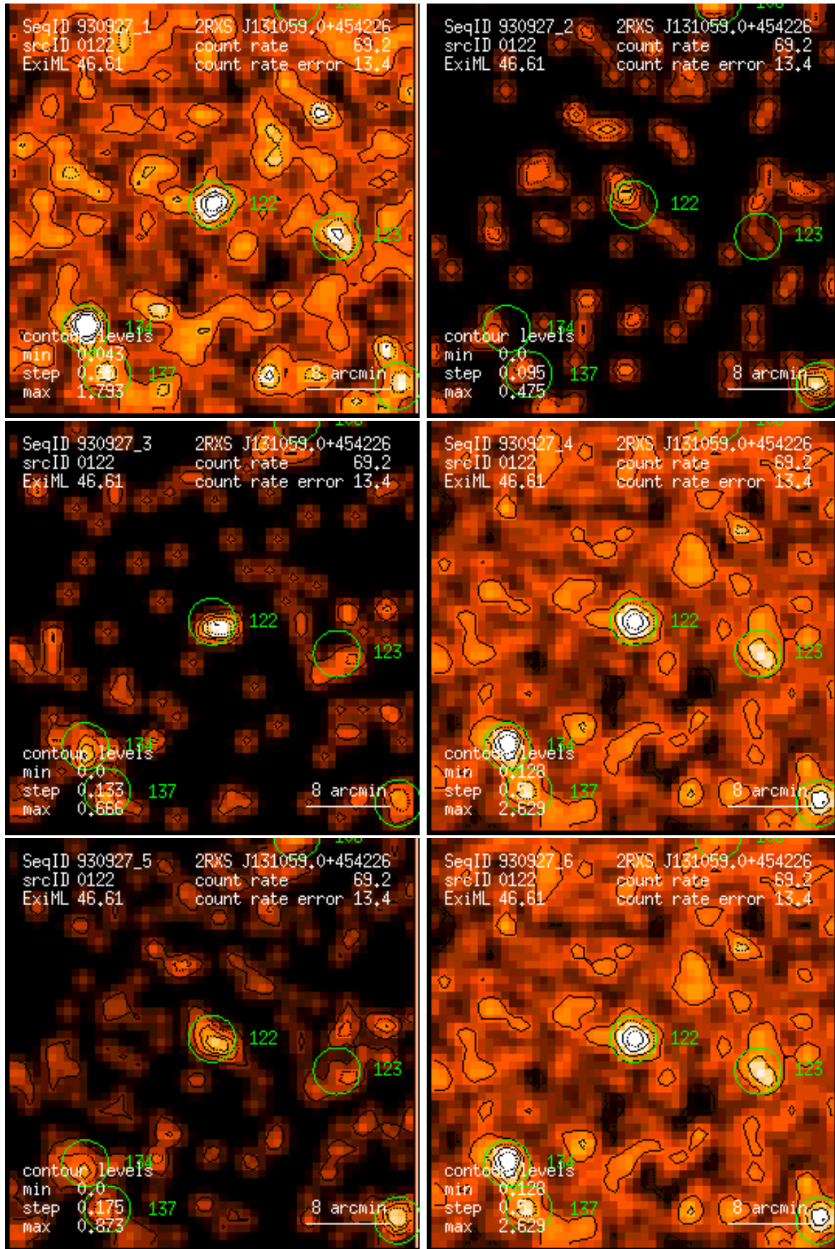
Figure 122: RASS 930927: detection 0122: band rate images, Gaussian filter: (1) PSPC channels 11 – 41, (2) 52 – 90, (3) 91 – 201, (4) 11 – 235, (5) 52 – 201, (6) 11 – 201. Broad band rates in counts/ks. Band rate contour levels in counts/ks/arcmin 2 .
