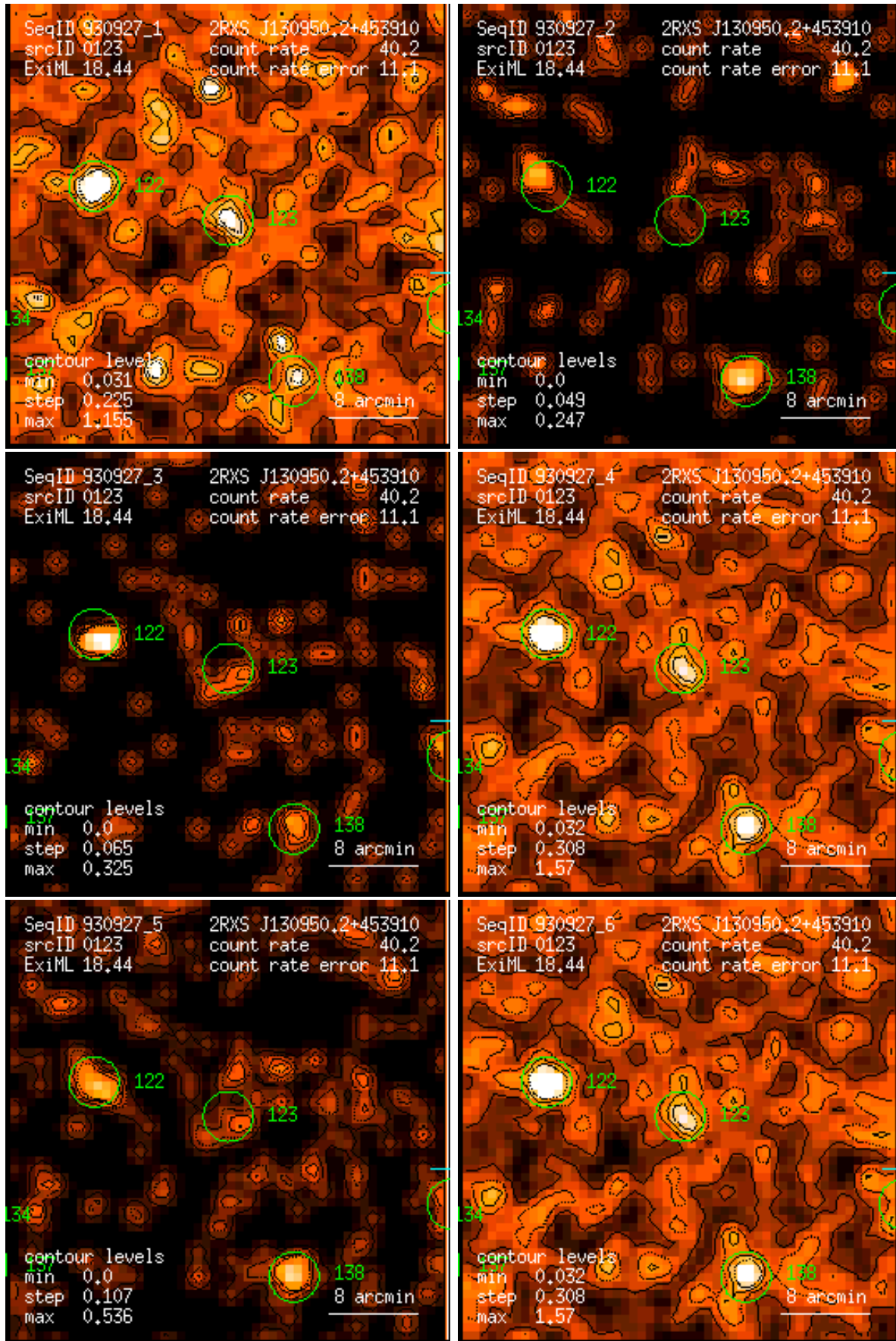
Figure 123: RASS 930927: detection 0123: band rate images, Gaussian filter: (1) PSPC channels 11 – 41, (2) 52 – 90, (3) 91 – 201, (4) 11 – 235, (5) 52 – 201, (6) 11 – 201. Broad band rates in counts/ks. Band rate contour levels in counts/ks/arcmin 2 .
