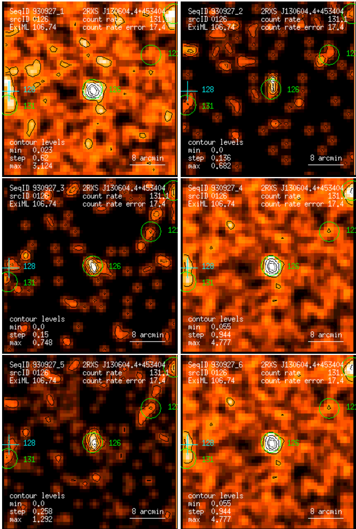
Figure 126: RASS 930927: detection 0126: band rate images, Gaussian filter: (1) PSPC channels 11 – 41, (2) 52 – 90, (3) 91 – 201, (4) 11 – 235, (5) 52 – 201, (6) 11 – 201. Broad band rates in counts/ks. Band rate contour levels in counts/ks/arcmin 2 .
