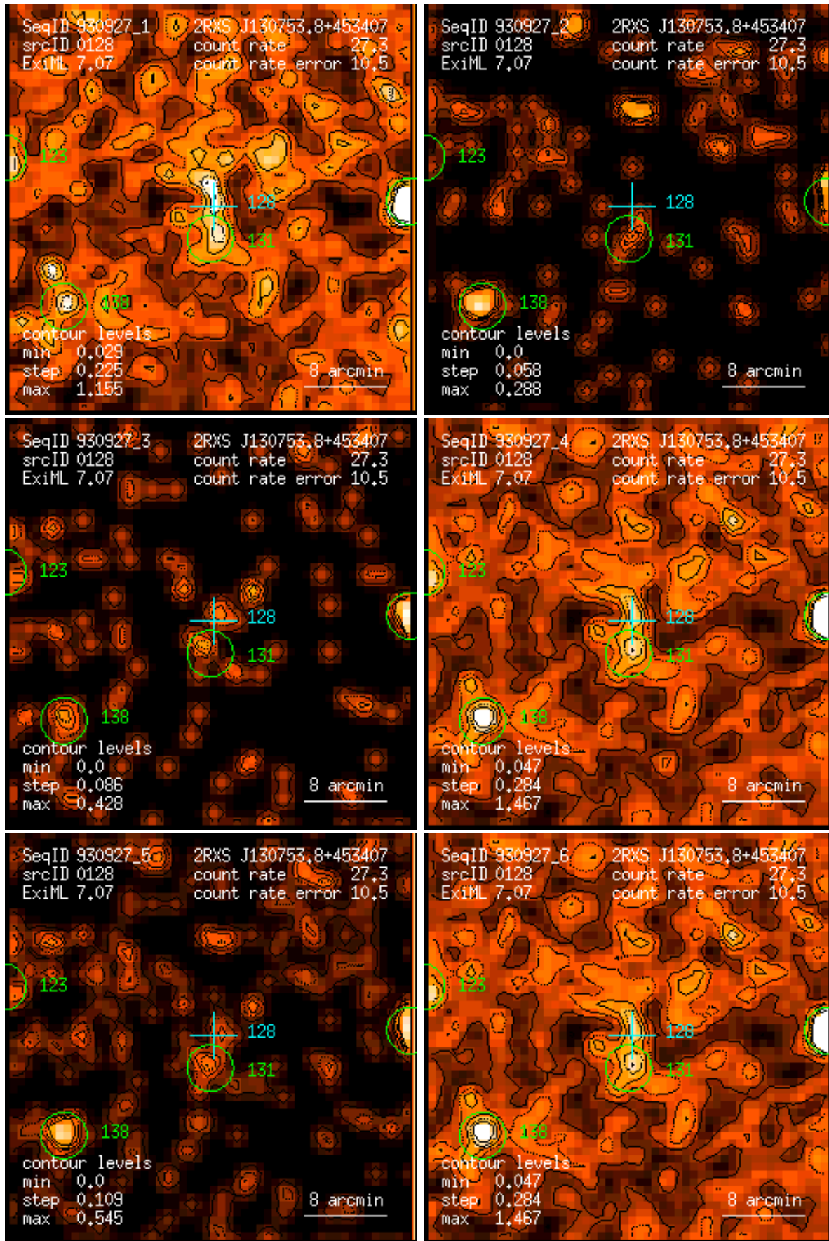
Figure 128: RASS 930927: detection 0128: band rate images, Gaussian filter: (1) PSPC channels 11 – 41, (2) 52 – 90, (3) 91 – 201, (4) 11 – 235, (5) 52 – 201, (6) 11 – 201. Broad band rates in counts/ks. Band rate contour levels in counts/ks/arcmin 2 .
