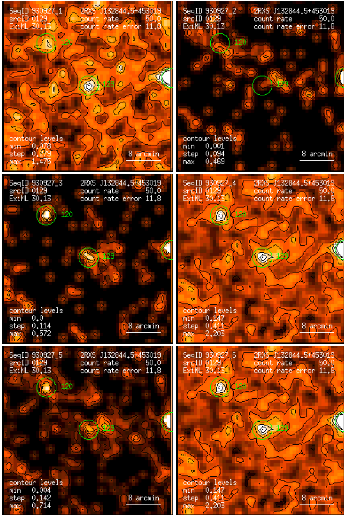
Figure 129: RASS 930927: detection 0129: band rate images, Gaussian filter: (1) PSPC channels 11 – 41, (2) 52 – 90, (3) 91 – 201, (4) 11 – 235, (5) 52 – 201, (6) 11 – 201. Broad band rates in counts/ks. Band rate contour levels in counts/ks/arcmin 2 .
