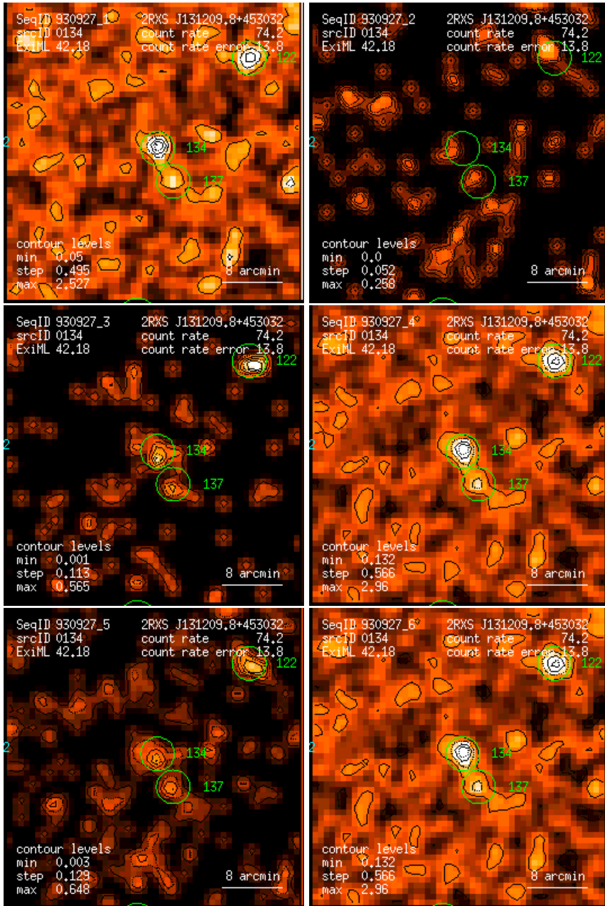
Figure 134: RASS 930927: detection 0134: band rate images, Gaussian filter: (1) PSPC channels 11 – 41, (2) 52 – 90, (3) 91 – 201, (4) 11 – 235, (5) 52 – 201, (6) 11 – 201. Broad band rates in counts/ks. Band rate contour levels in counts/ks/arcmin 2 .
