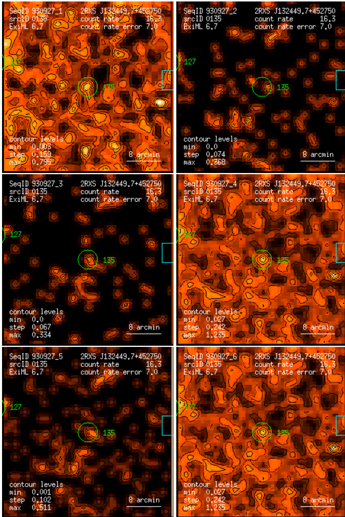
Figure 135: RASS 930927: detection 0135: band rate images, Gaussian filter: (1) PSPC channels 11 – 41, (2) 52 – 90, (3) 91 – 201, (4) 11 – 235, (5) 52 – 201, (6) 11 – 201. Broad band rates in counts/ks. Band rate contour levels in counts/ks/arcmin 2 .
