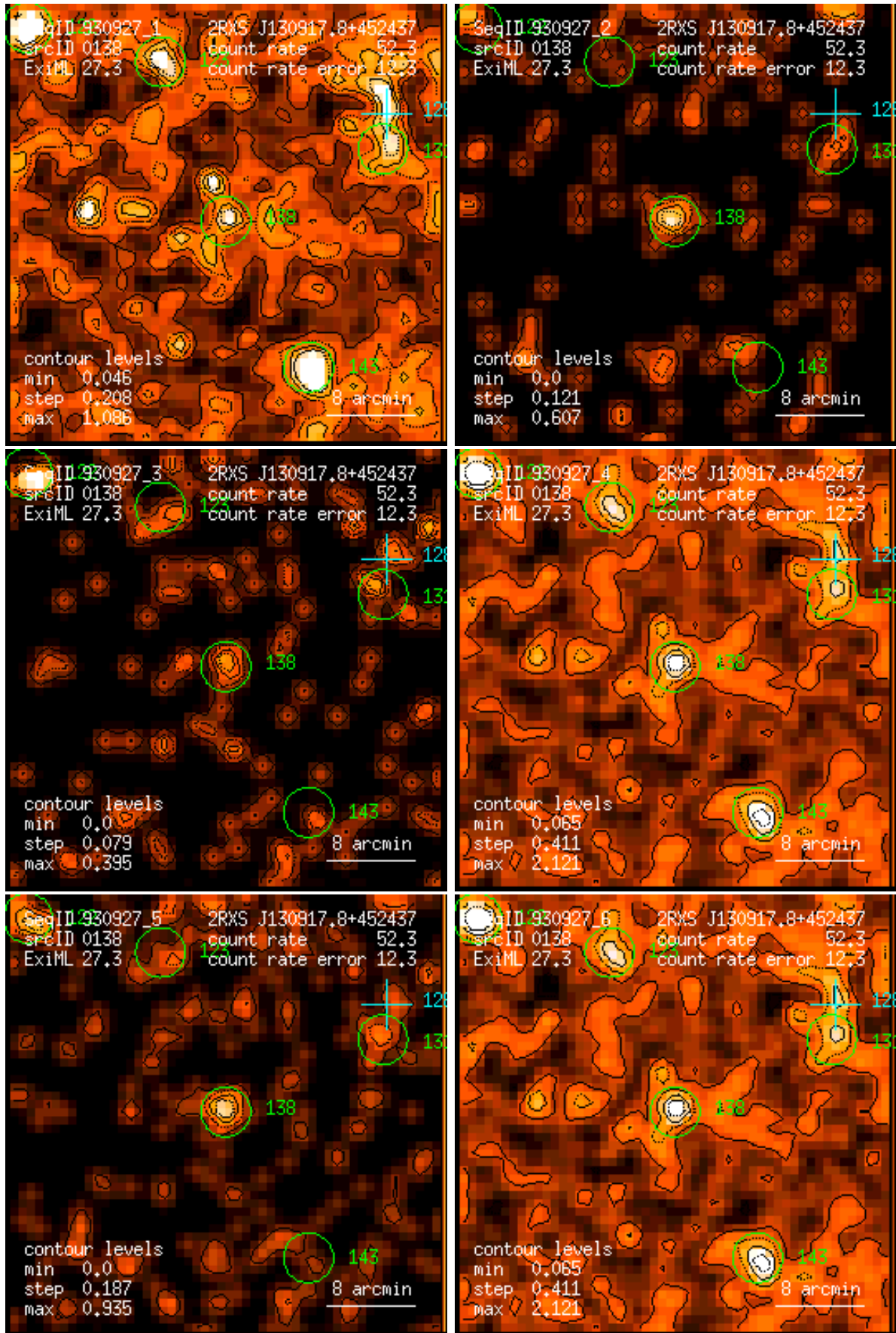
Figure 138: RASS 930927: detection 0138: band rate images, Gaussian filter: (1) PSPC channels 11 – 41, (2) 52 – 90, (3) 91 – 201, (4) 11 – 235, (5) 52 – 201, (6) 11 – 201. Broad band rates in counts/ks. Band rate contour levels in counts/ks/arcmin 2 .
