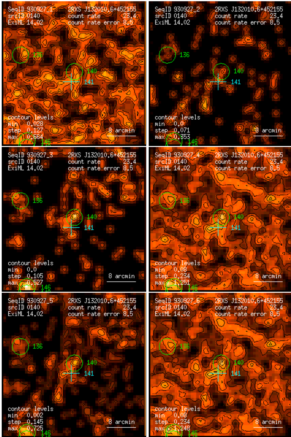
Figure 140: RASS 930927: detection 0140: band rate images, Gaussian filter: (1) PSPC channels 11 – 41, (2) 52 – 90, (3) 91 – 201, (4) 11 – 235, (5) 52 – 201, (6) 11 – 201. Broad band rates in counts/ks. Band rate contour levels in counts/ks/arcmin 2 .
